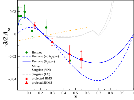
Figure 7: NEEDS TO BE UPDATED. Corresponding projected precision of the tensor asymmetry A_{zz} . Data at different Q^2 are combined with an x-binning that varies slightly per point, but is approximately \pm 0.05 . The black band represents the systematic uncertainty. Also shown are the HERMES data [9], and the calculations from Kumano [12], Miller [13, 14], and Sargsian [17].
