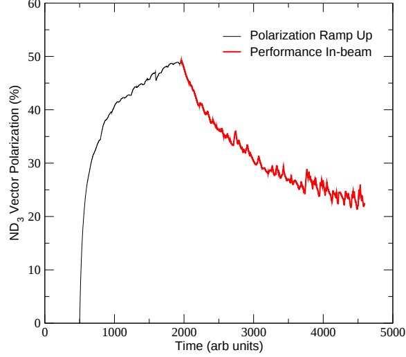
Figure 11: Performance of the \text{ND}_3 target during the GeN experiment.
