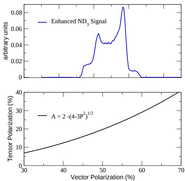
Figure 10: Top: NMR signal for \text{ND}_3 with a vector polarization of approximately 50% from the GeN experiment. Bottom: Relationship between vector and tensor polarization in equilibrium, and neglecting the small quadrupole interaction.
