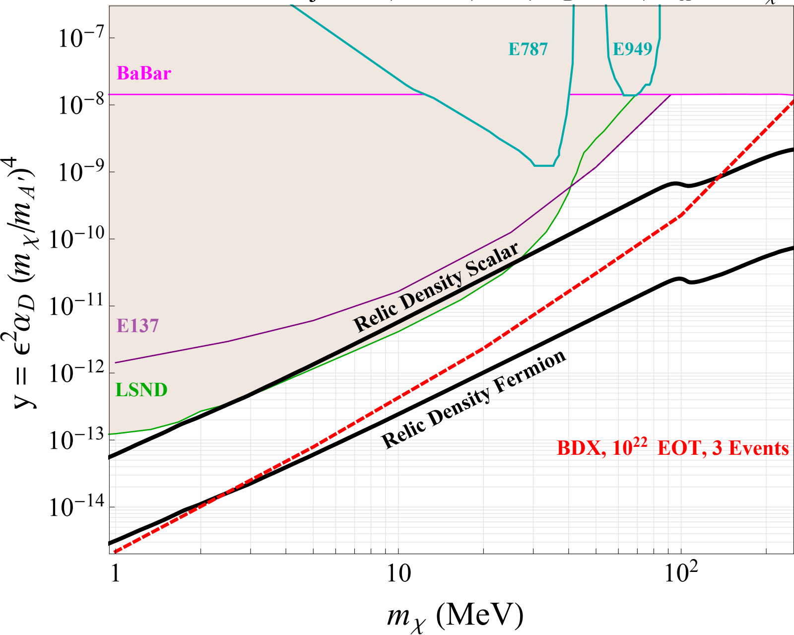
Thermal Relic Majorana (Inelastic) DM, \alpha_D = 0.1 , m_{A'} = 3 m_\chi
