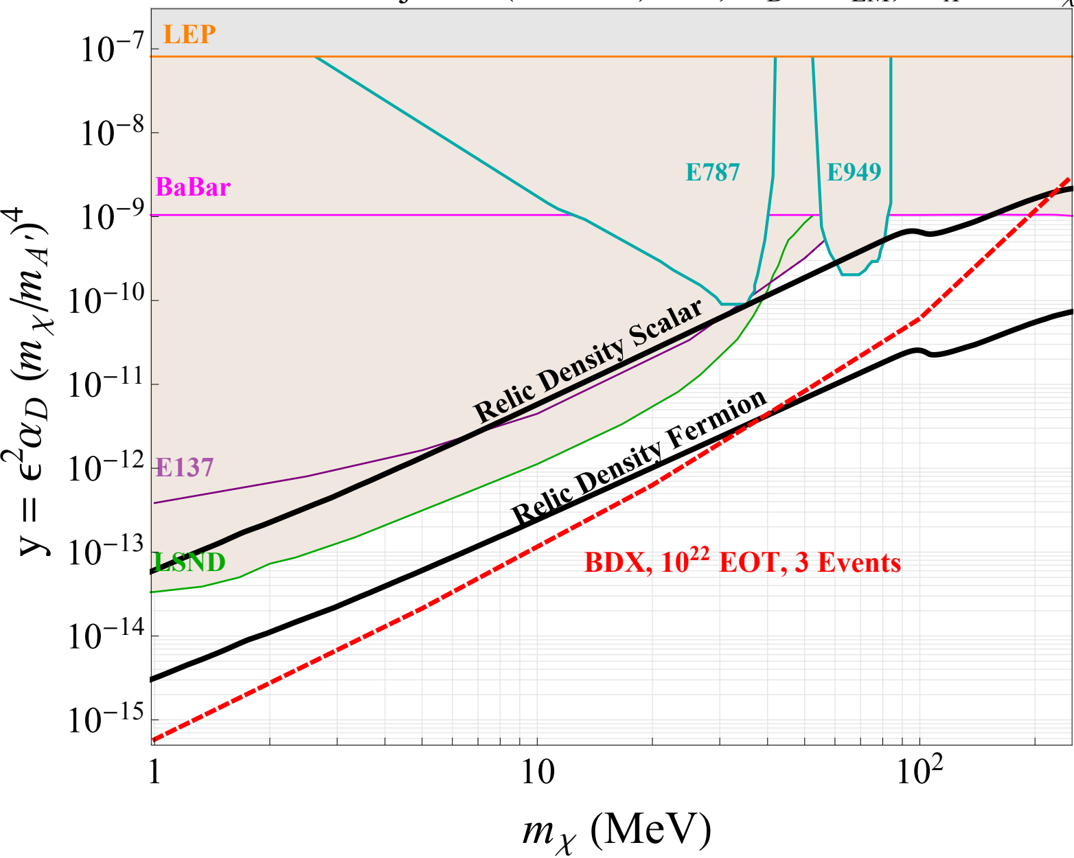
Thermal Relic Majorana (Inelastic) DM, \alpha_D = \alpha_{\text{EM}} , m_{A'} = 3 m_\chi
