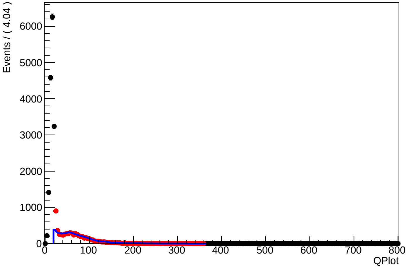
A RooPlot of "QPlot"
