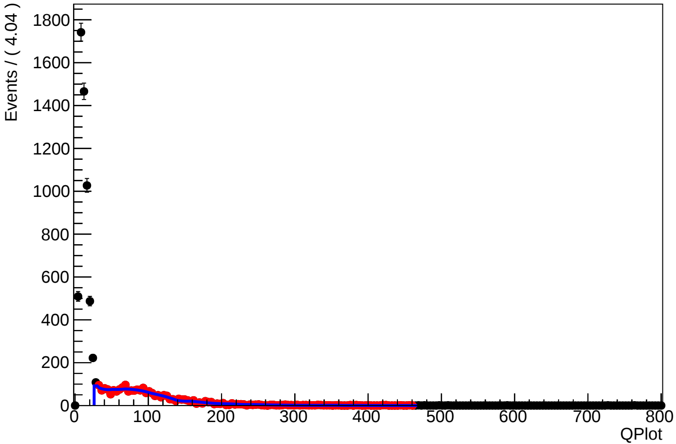
A RooPlot of "QPlot"
