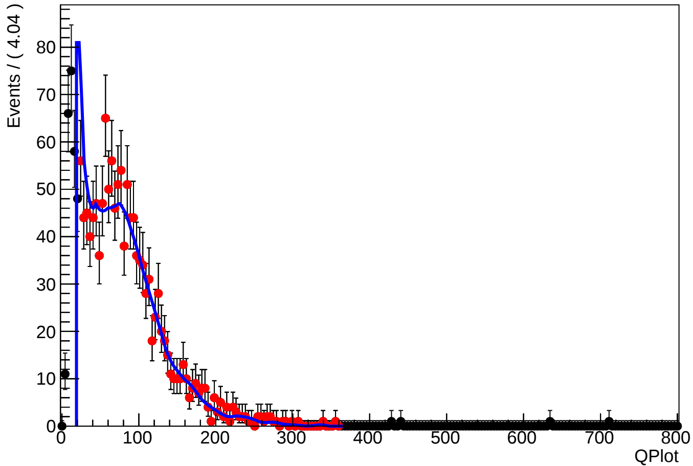
A RooPlot of "QPlot"
