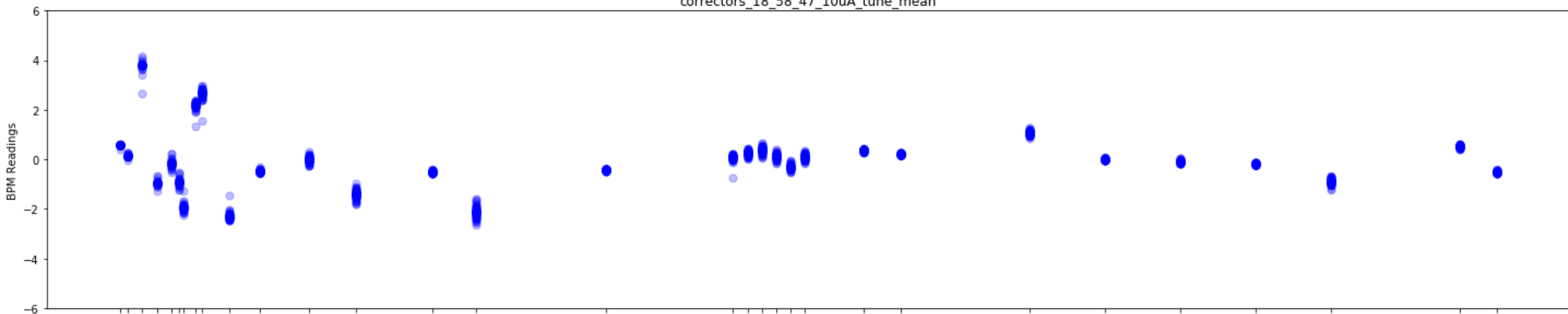
Vertical BPM Readings for BASE Settings: correctors_18_58_47_10uA_tune_mean
