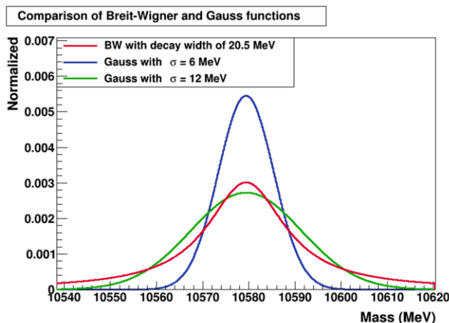
Y(4S) resonance and collision energy spreads w/o and with moderate monochromatization ( \lambda=2 ) [Courtesy Andreas Hoecker (spokesperson of ATLAS), on the flight from Narita to Zürich].
