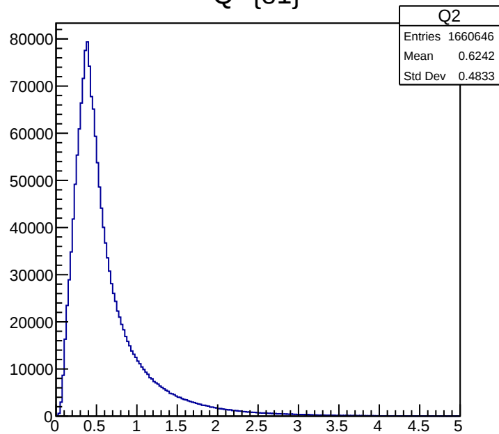
Q^2 \{e1\}
