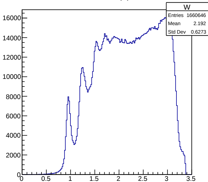
W = MM(e)
