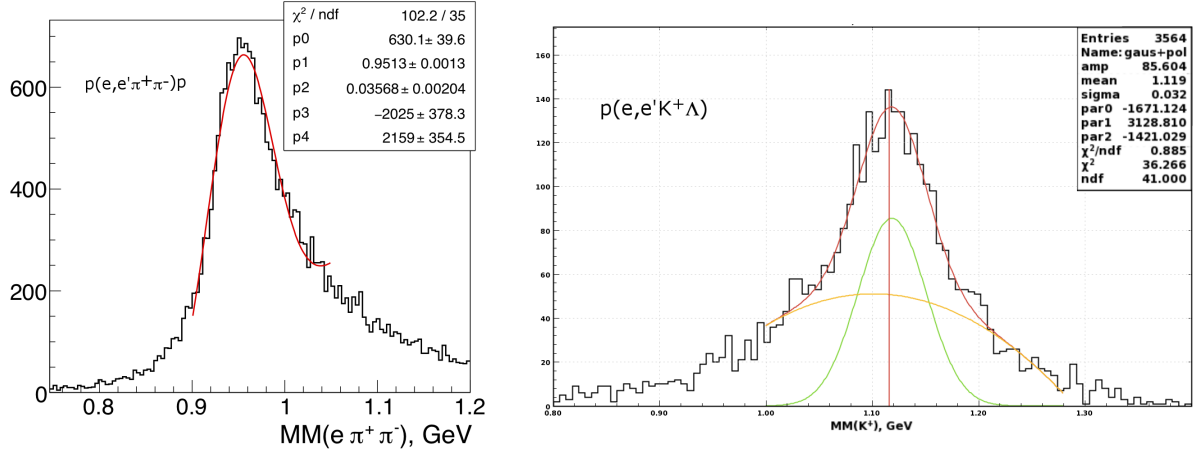
Figure 3: Left plot: Preliminary e'\pi^+\pi^- missing mass distribution for the \pi^+\pi^-p exclusive channel for electrons detected in the CLAS12 Forward Detector at 6.5 GeV electron energy. Right plot: Preliminary e'K^+ missing mass distribution for the K^+\Lambda exclusive channel for electrons detected in the Forward Tagger. The analyzed data correspond to about 5% of the 7.5 GeV RG-K Fall 2018 data.
