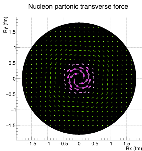
Figure 2: Distribution of shear forces in the proton extracted from a model for the Compton Form Factor \mathcal{H} . The shear stress changes direction at a radial value of 0.5 fm, which constrains the integrated torque to be equal 0.
