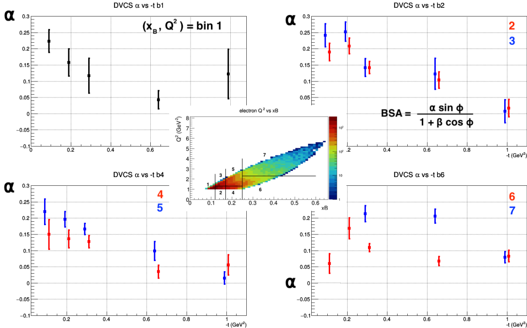
Figure 5: Preliminary DVCS beam spin asymmetries amplitudes as a function of t for all (x_B, Q^2) bins.
