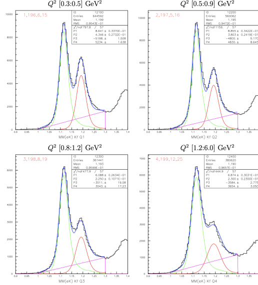
Figure 4: Preliminary e'K^+ missing mass distributions (with the K^+ detected in the Forward Detector) from 9 runs of the 6.5 GeV RG-K data set before final calibrations and without momentum corrections as a function of Q^2 showing the spectrum fits used for the yield extraction of the K^+\Lambda and K^+\Sigma^0 final states.
