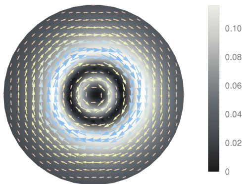
Figure 2: Distribution of shear forces in the proton extracted from a model for the Compton Form Factor \mathcal{H} . The shear stress changes direction at a radial value of 0.5 fm, which constrains the integrated torque to be equal 0. Figure taken from Ref. [4]. The radius of the disc in the figure is 1.5 fm and the color scale gives the absolute value of the tangential force in GeV/fm.
