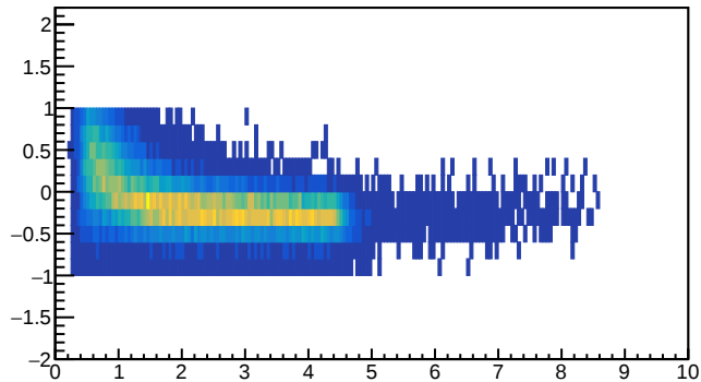
FT Electron \Delta T V P
