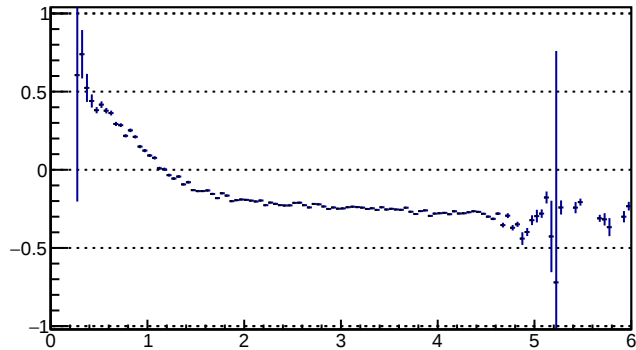
Fit Mean V P
