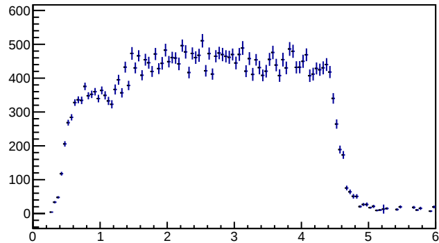
Fit Height V P
