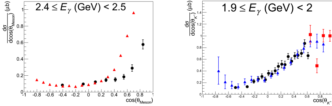
(a) CLAS g13 \gamma D \rightarrow K^*(892)^0\Lambda(p) (black circles) and CLAS g11 \gamma p \rightarrow K^+\Lambda (red triangles). No data available for \gamma D \rightarrow K^0\Lambda(p) .
