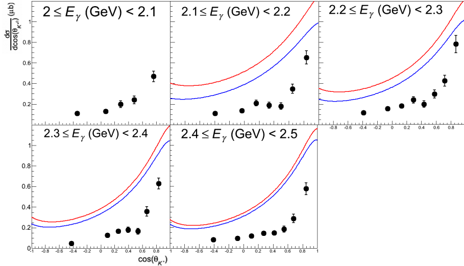
Figure 2: For \gamma D \rightarrow K^*(892)^0 \Lambda(p) , the preliminary CLAS g13 (black circles) differential cross section data and the model predictions by Kim et al. [11] with (red) and without (blue) N^* resonances in the model.
