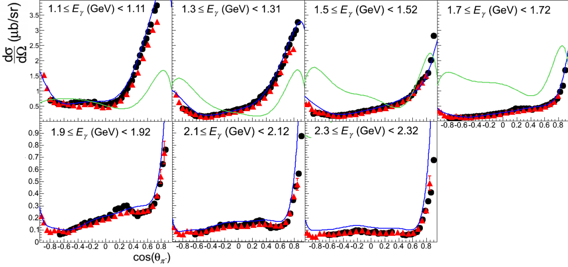
Figure 1: For \gamma D \rightarrow p\pi^-(p) , the preliminary CLAS g13 (black circles) and CLAS g10 [7] (red triangles) differential cross section data, and the SAID GB11 (blue) [8] and Bonn Gatchina BnGa12-1 [10] (green) predictions. The statistical uncertainties are smaller than the data markers.
