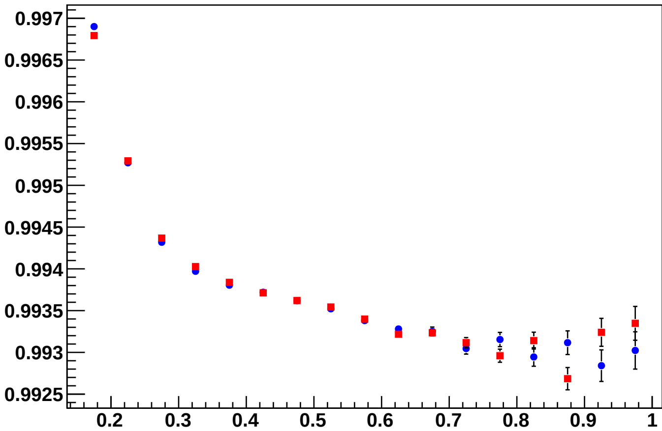
Mean Value of cosphi Per X Bin
