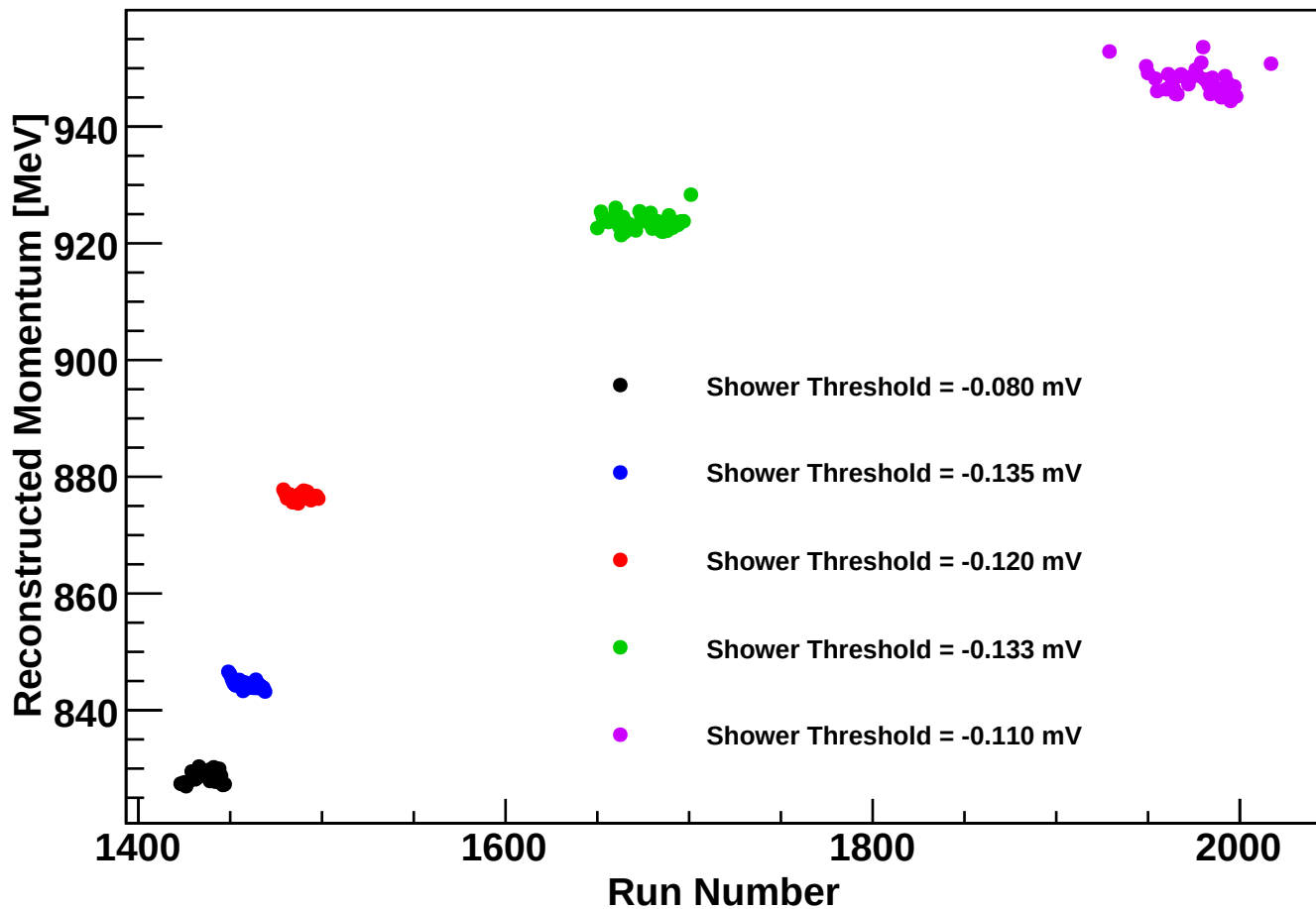
Mean Reconstructed Momentum for 5.89 GeV, S = 90°
