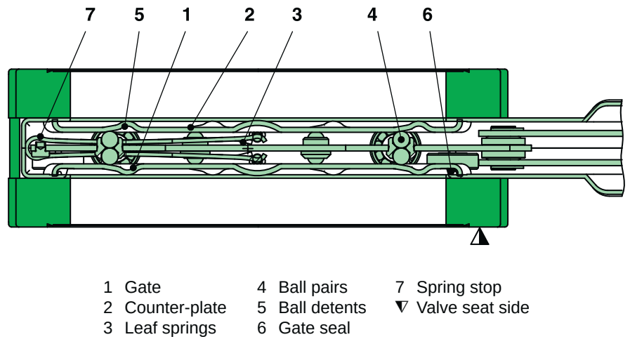
Functional principle
