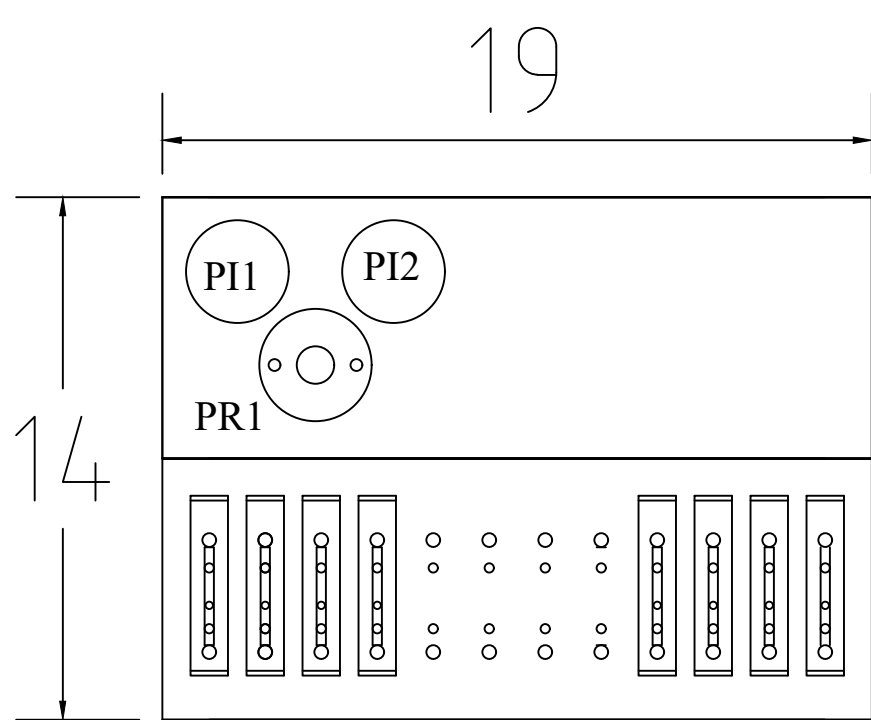
Hall A GEM BB Gas Distribution FRONT Panel
