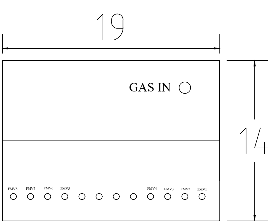
Hall A GEM BB Gas Distribution REAR Panel
