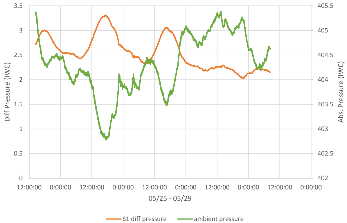
S1 Pressure vs. Amb. Pressure
