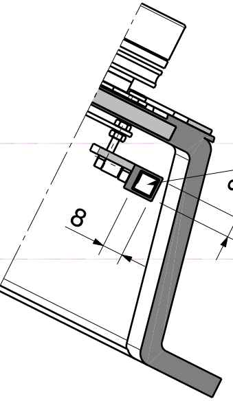
Section view B-B Scale: 1:2
