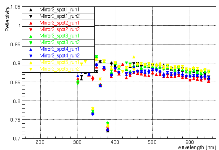
Reflectivity
