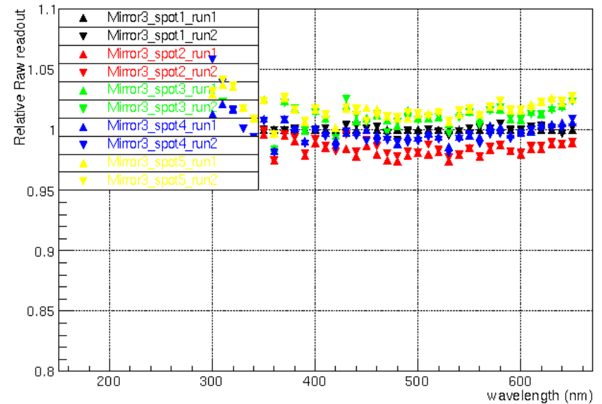
Reflectivity
