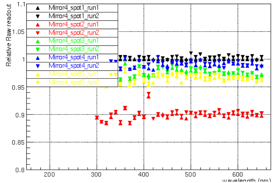
Reflectivity
