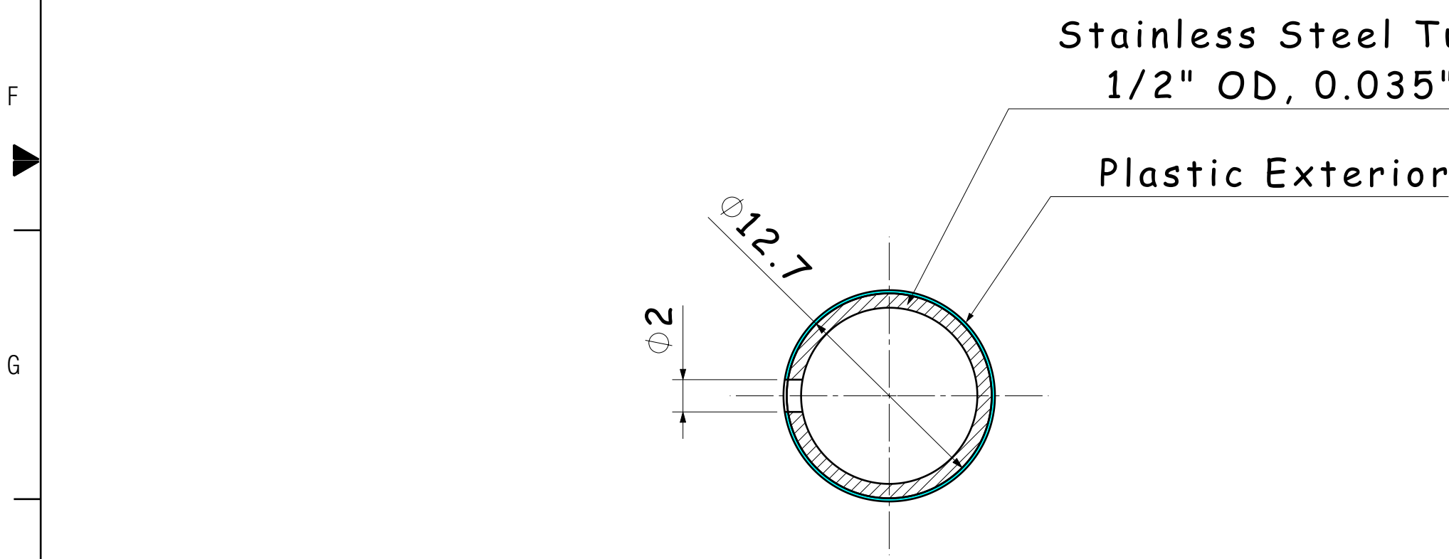
Section view B-B Scale: 3:1
