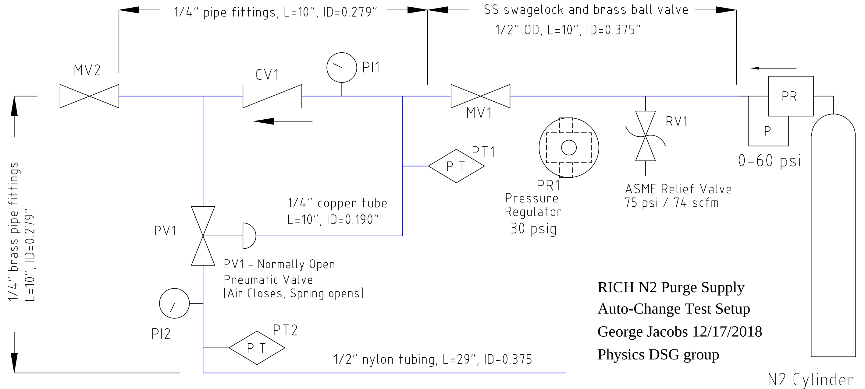
RICH N2 Gas Supply Auto-Change Test Setup
