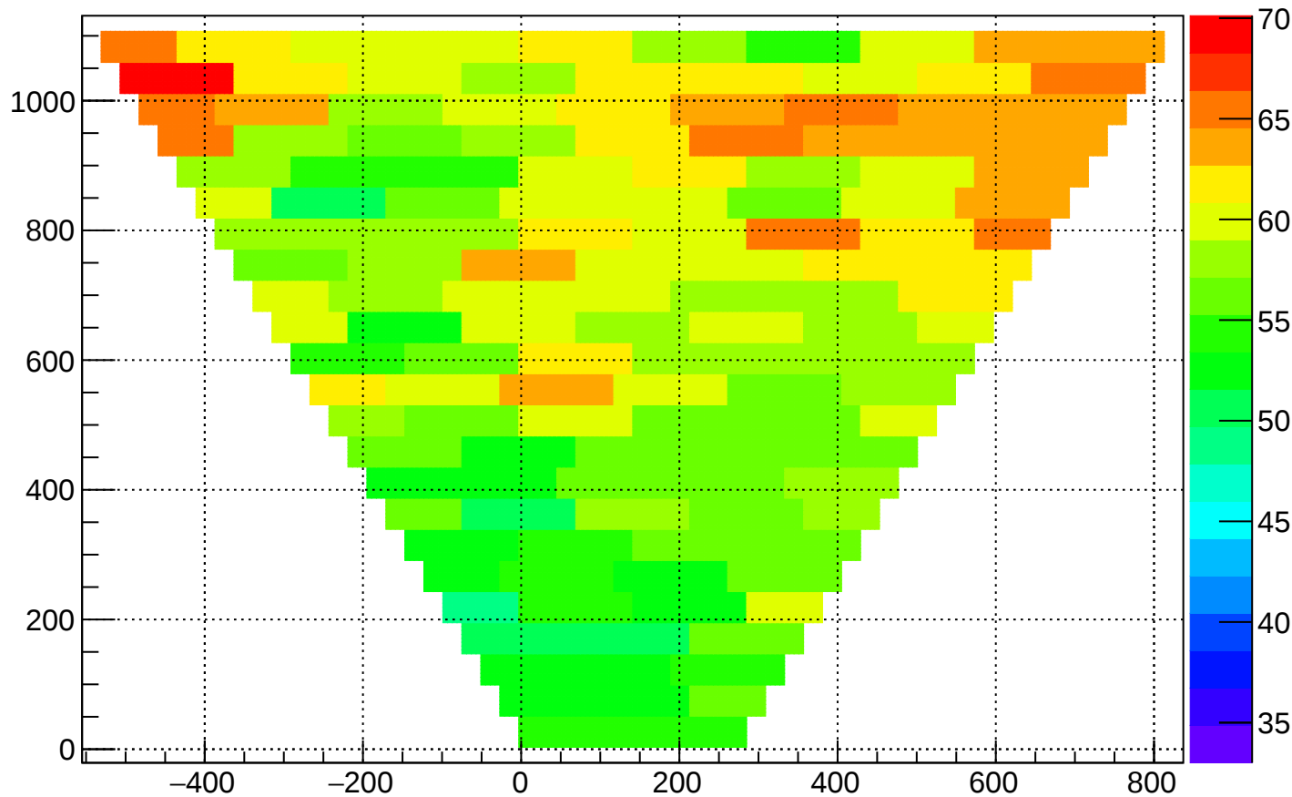
FPGA Temperature map, T=151140.0 sec
