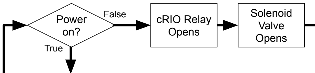
Power Loss Process Diagram
