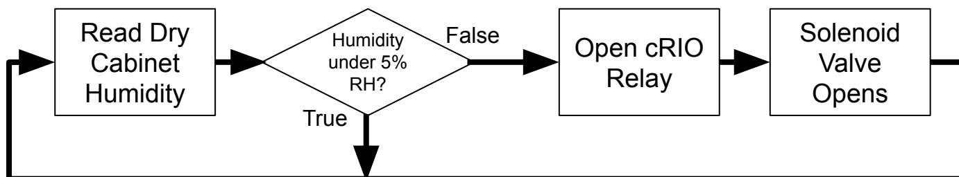
Aerogel Humidity Interlock Process Diagram
