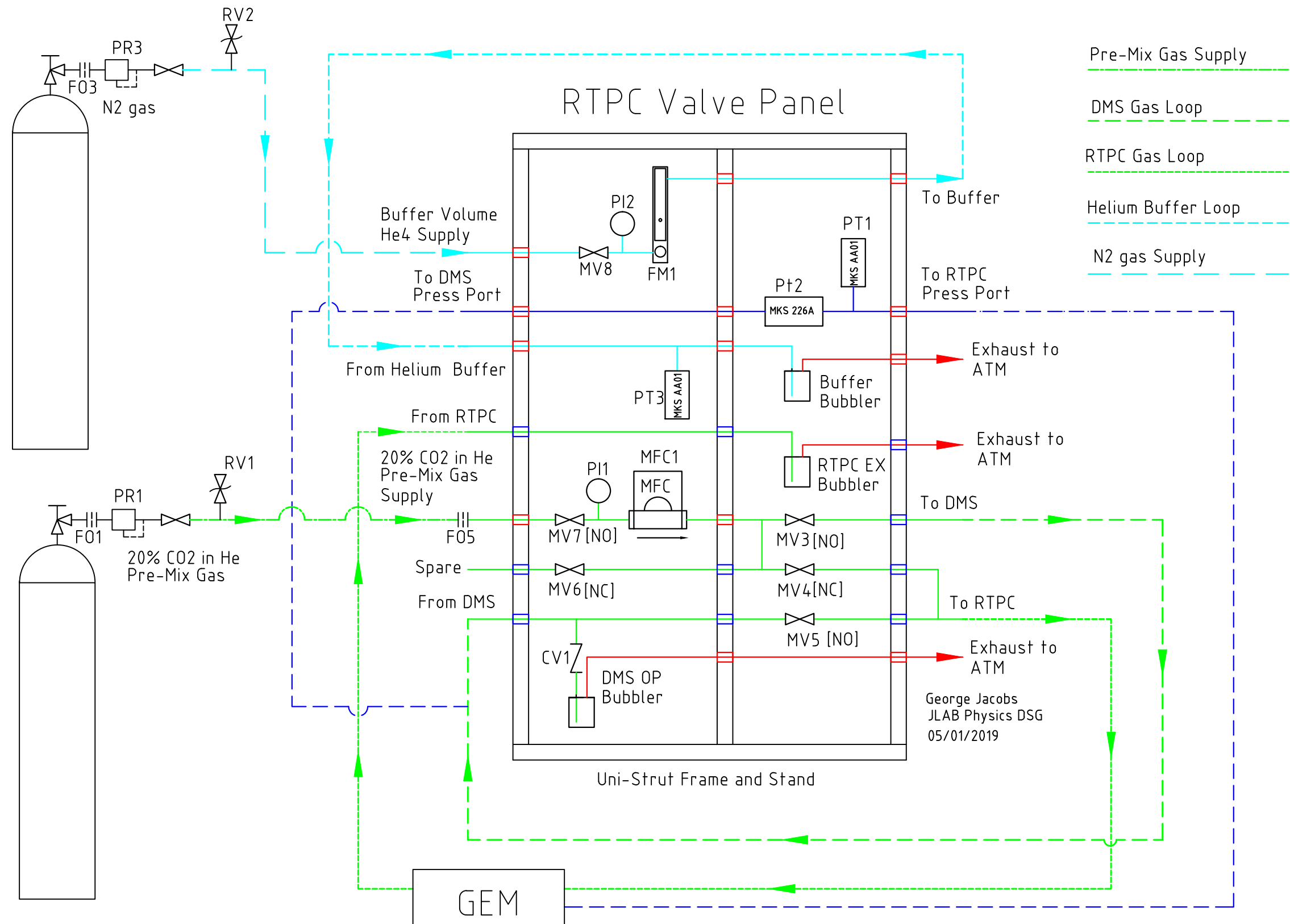
RTPC Valve Panel Testing with GEM Detector – EEL rm125
