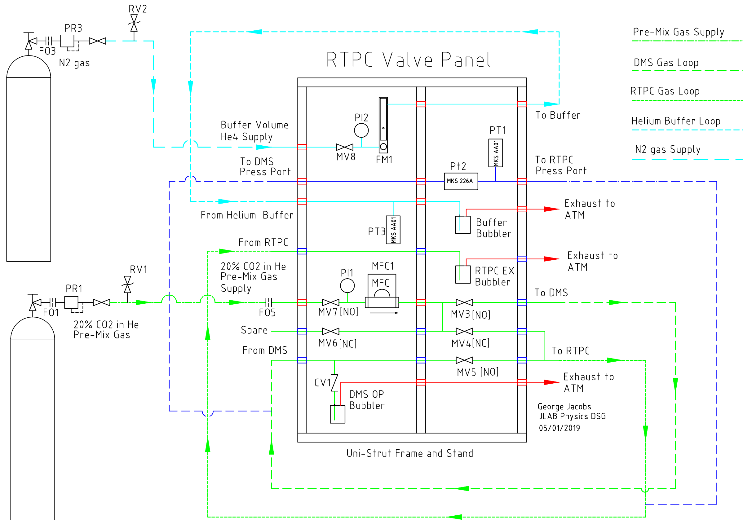
RTPC Valve Panel Component Testing Connections - EEL rm125
