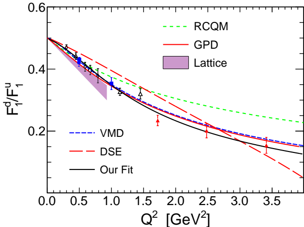
FIG. 2: Nucleon flavor FF ratio F_1^d/F_1^u vs Q^2 . The band indicates the lattice QCD result [34]. Data and curves are the same as in Fig. 1.
