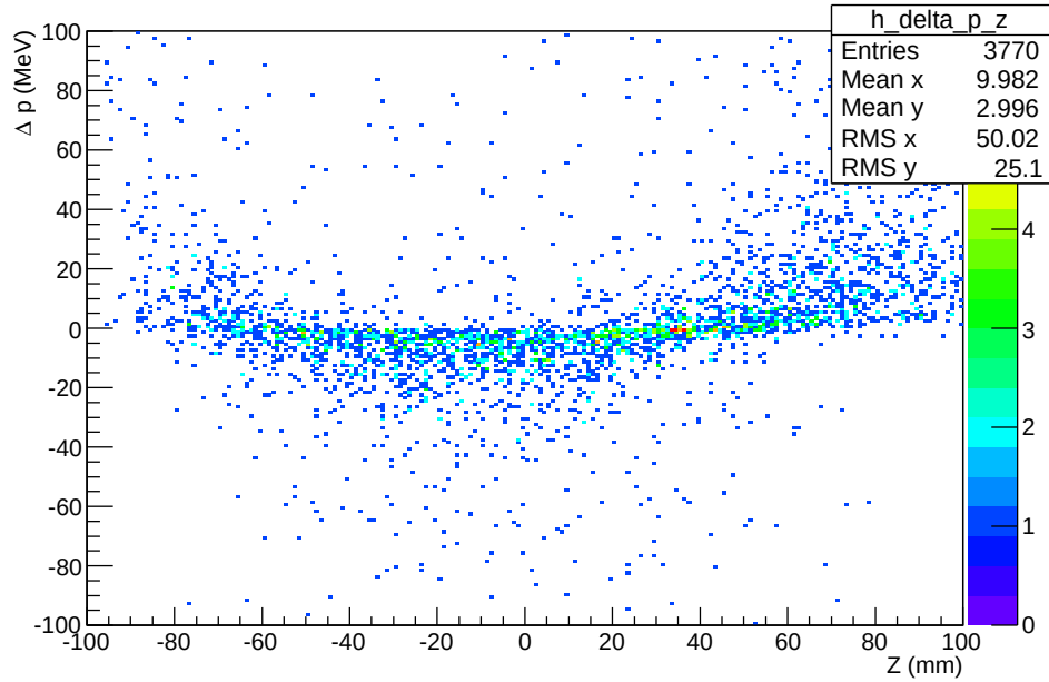
delta_p vs. Z
