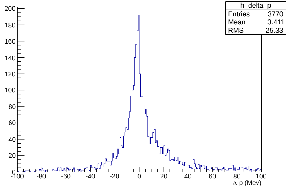
P difference for the overlap events
