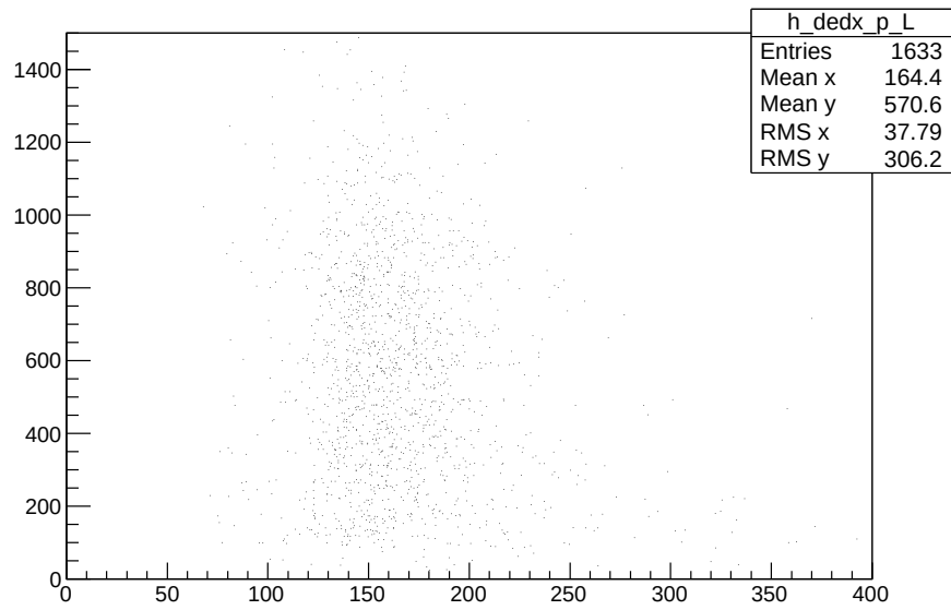
dE/dx vs. P with -60 < z < 80 left side
