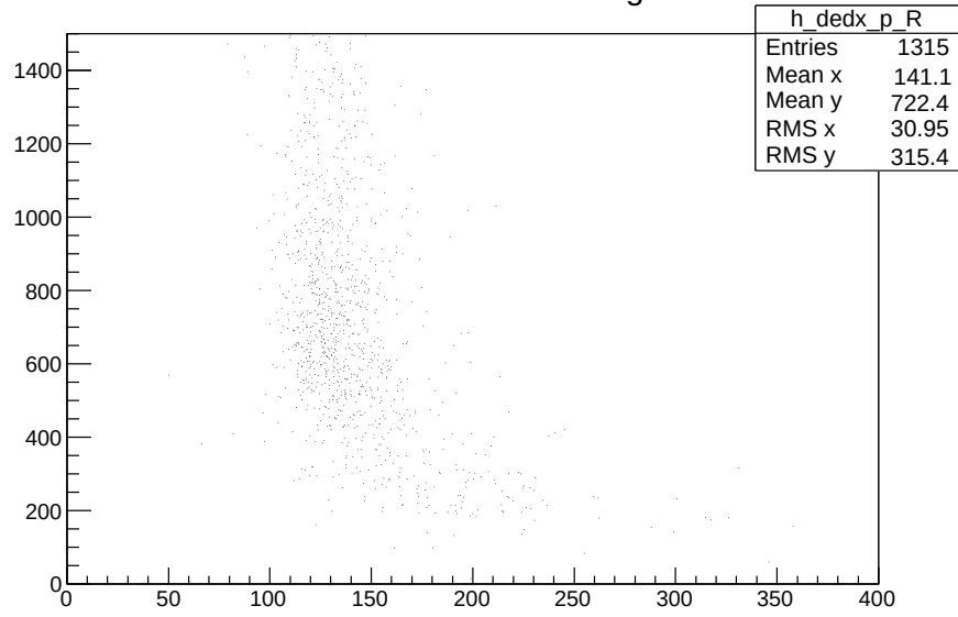
dE/dx vs. P with -60 < z < 80 right side
