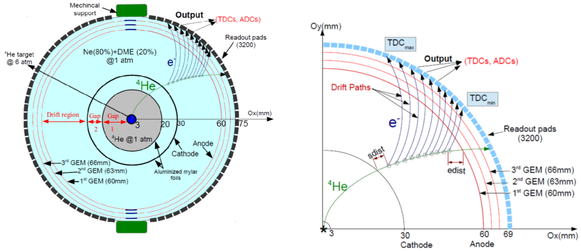
(a) Schematic of ^4\text{He} track, in green, with ionized electrons, in dark blue, in RTPC (b) Zoomed quadrant of RTPC with GEM layers and readout pads shown
