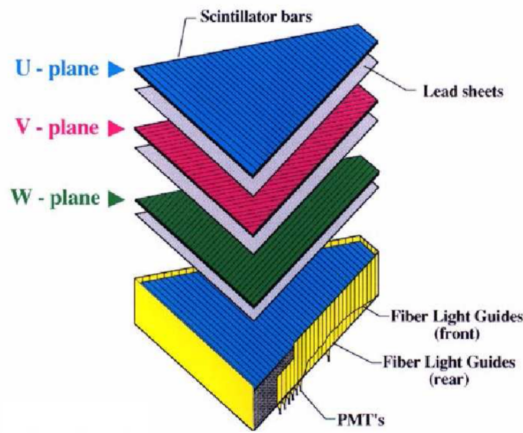
Figure 3.7: The layers of the EC [3]
