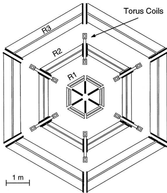
Figure 3.4: The torus embedded inside the DC, extending from the 2nd DC region to 3rd [24].
