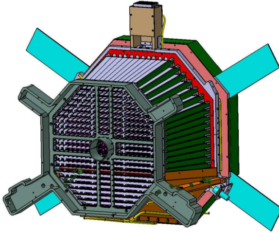
Figure 4.2: The IC represented in GEANT [25]
