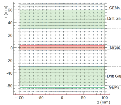
Figure 4.5: Profile view of the magnetic field map in the RTPC produced by the solenoid [3]
