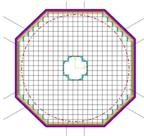
(b) Schematic of crystal array for IC [25]
