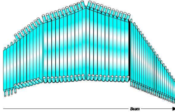
Figure 3.6: Profile view of a sector of the SC: Pictured are the 57 scintillator strips and PMTs on each end of the strips. [3]
