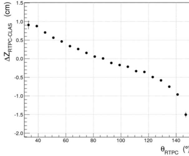
Figure B.2: RTPC Vertex Correction: \Delta z vs \theta showing a linear dependence [33].
