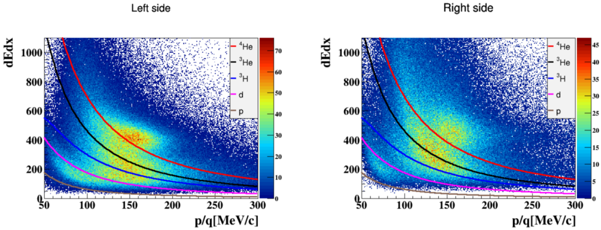
Figure 7.7: Bethe-Bloch curves overlaying the dE/dx vs. p/q distributions for the left and right sides of the RTPC [3].
