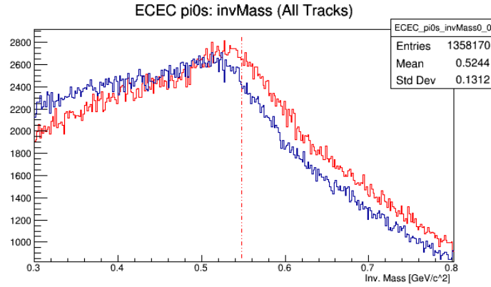
Figure B.17: Invariant mass distribution generic EC photon pairs. The blue and red are the uncorrected and corrected distributions, respectively. The red is the nominal value of the \eta invariant mass.
