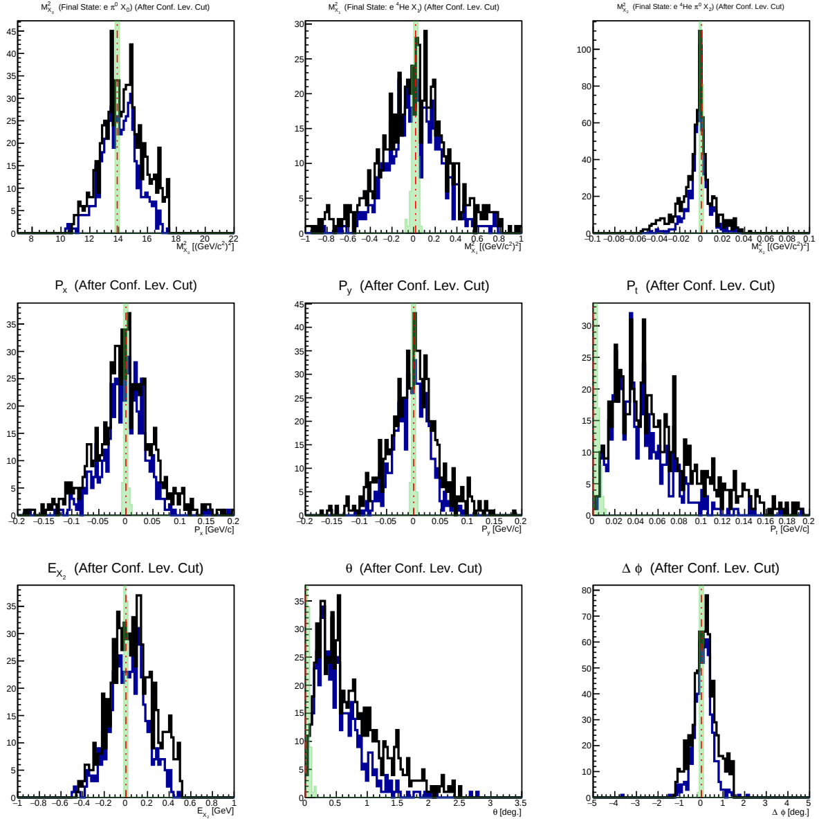
Figure 14.3: Exclusivity variable distributions for:
