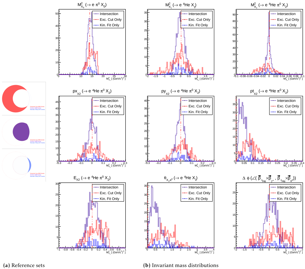
Figure 15.8: Exclusivity variable distributions of the disjoint sets:
