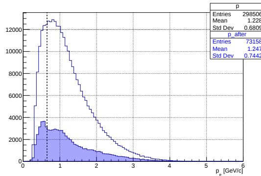
Figure 5.5: Momentum cut: To protect against Møller electrons and \pi^- a cut on the momentum is applied.
