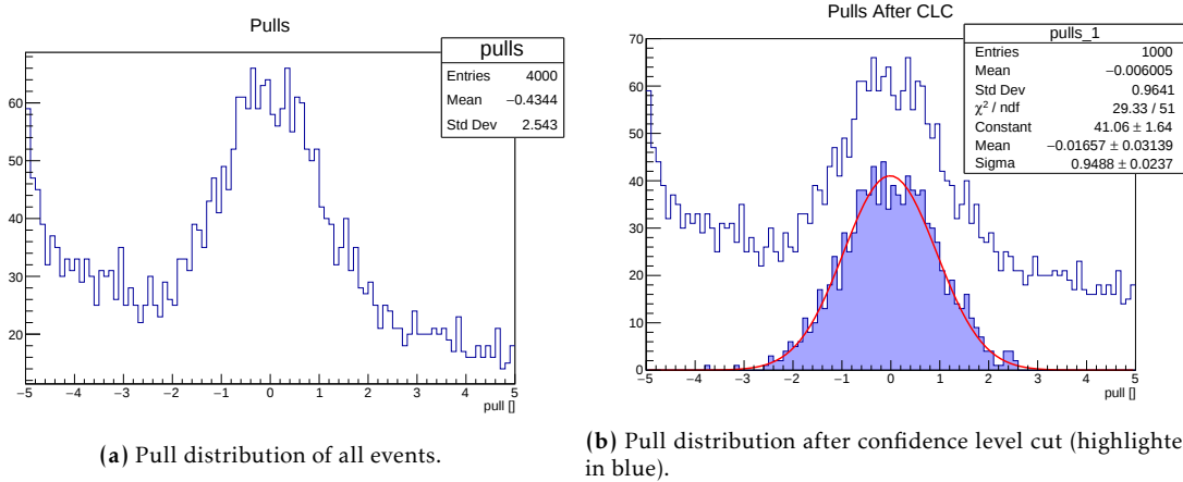
Figure 10.3: Pull distribution before (left) and after (right) confidence level cut.
