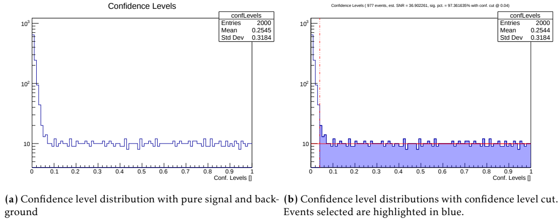
Figure 10.2: Confidence level distributions before (left) and after (right) CLC.
