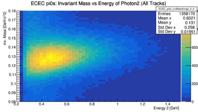
Figure B.9: Invariant mass of two EC photons vs. energy of the lower energy photon : The peak of the invariant mass is dependent on the energy of the lower energy photon.
