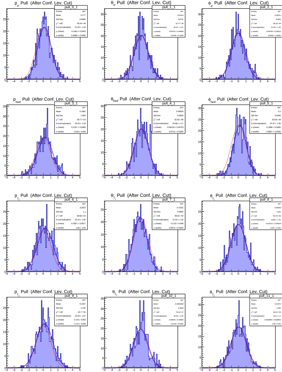
Figure 14.2: Pull distributions. From left to right we have p, \theta, \phi of the, from top to bottom, particles e, ^4\text{He}, \gamma_1, \gamma_2 . The blue curve is a gaussian fit to the distribution. The red curve is just a visual aid of what the distribution should be: a gaussian normalized to the blue curve with width 1, centered at 0.
