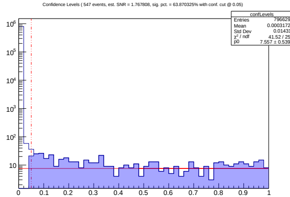
Figure 14.1: Confidence level distribution with a cut at 0.05, represented by the red vertical dashed line. The events passing the cut are represented by the light blue highlighted distribution which the right half is fitted to straight line to estimate the signal to noise ratio.
