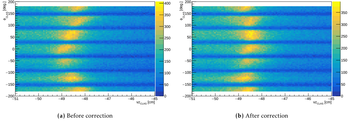
Figure B.1: Vertex Correction: An azimuthal angle dependent vertex shift is implemented to account for changes in beam position.
