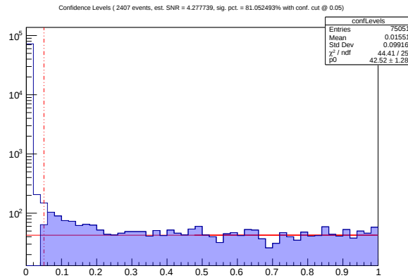
Figure 12.1: Confidence level distribution with a cut at 0.05, represented by the red vertical dashed line. The events passing the cut are represented by the light blue highlighted distribution which the right half is fitted to straight line to estimate the signal to noise ratio.
