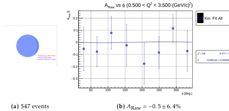
Figure 15.4: Beam spin asymmetry (b) of selected events (a): All events passing kinematic fitting
