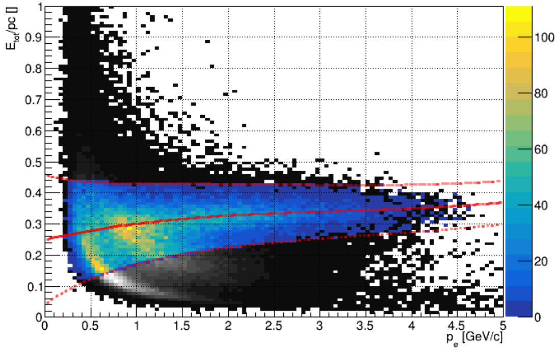
Figure 5.8: EC Sampling Fraction Cut: The distributions of the energy and sector dependent EC sampling fraction as a function of momentum are shown (for sector 1). The dependence is fitted and measurements 3.5 \sigma outside the fit are rejected (shown in red).
