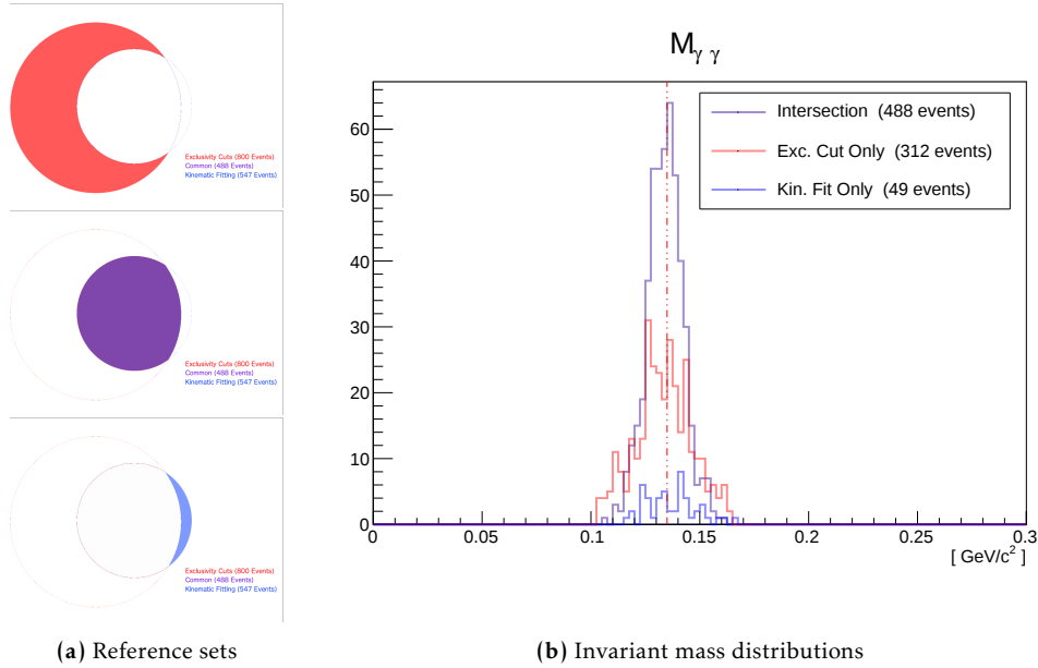
Figure 15.7: Invariant mass distributions of the disjoint sets: passing exclusivity cuts only, common events, and kinematic fitting only
