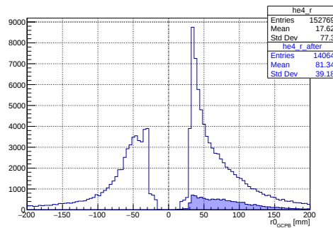
Figure 7.1: Charge Cut: Negatively charged tracks (negative radius of curvature) are thrown out.
