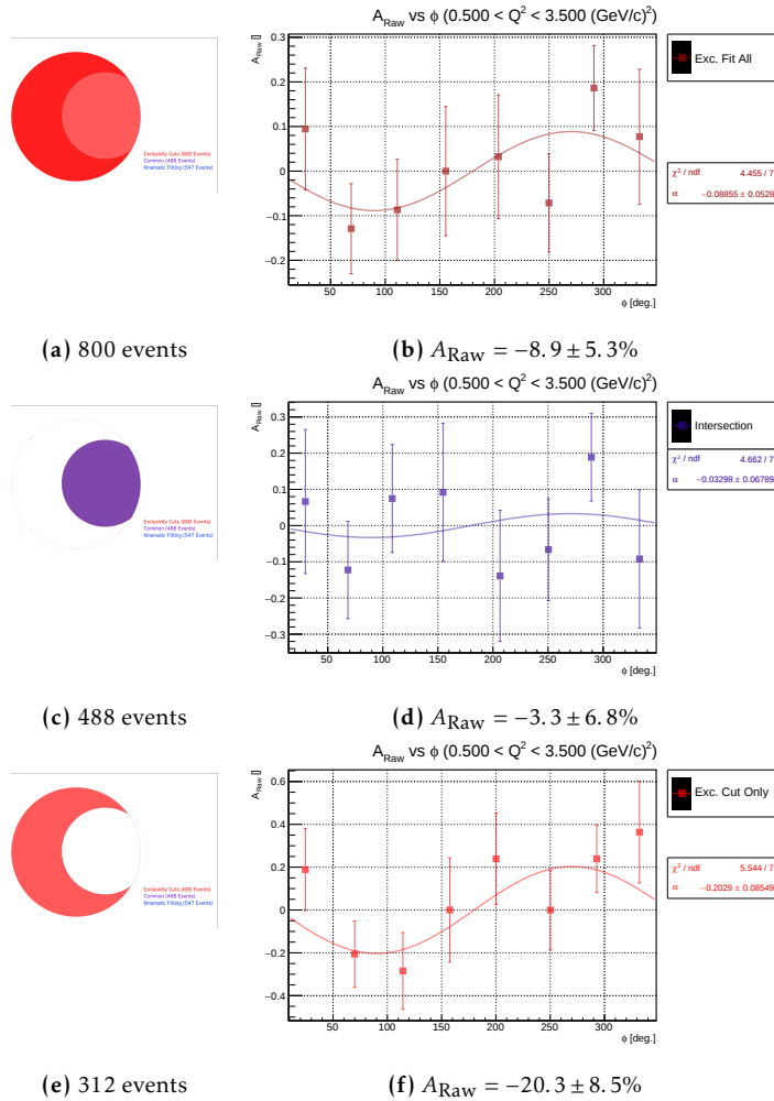
Figure 15.9: Beam spin asymmetries of selected events:
