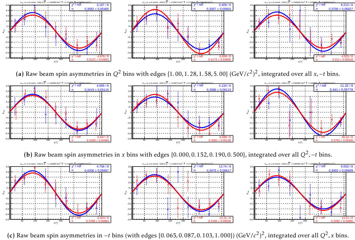
Figure 12.4: Raw beam spin asymmetry (Figs. 12.4a, 12.4b, 12.4c) for:
