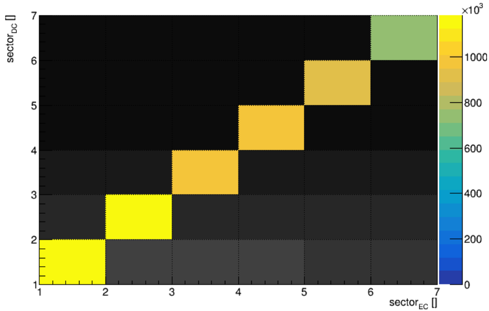
Figure 5.2: DC sector vs. EC sector: Only matching sectors will pass this cut.
