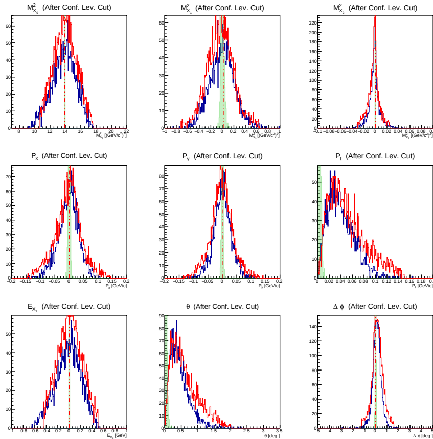
Figure 12.3: Exclusivity variable distributions for:
