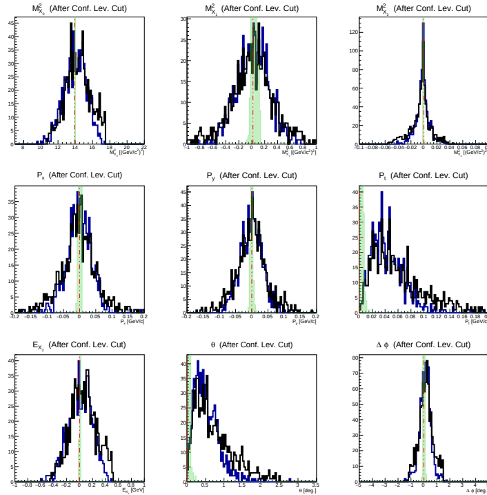
Figure 13.3: Exclusivity variable distributions for: - Measured events passing exclusivity cuts (black) - Measured events passing kinematic fit with 0.05 conf. level cut (blue) - Fitted events passing kinematic fit with 0.05 conf. level cut (highlighted green)
