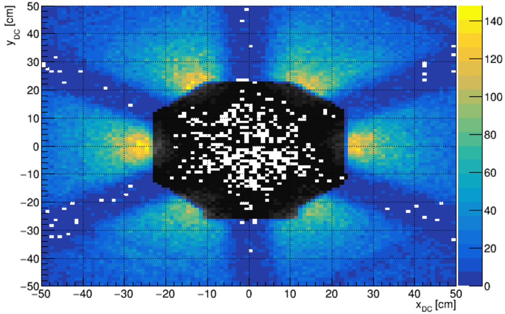
Figure 5.6: DC Fid. Cut: Tracks directly coming from the IC have energy loss that is unaccounted for.
