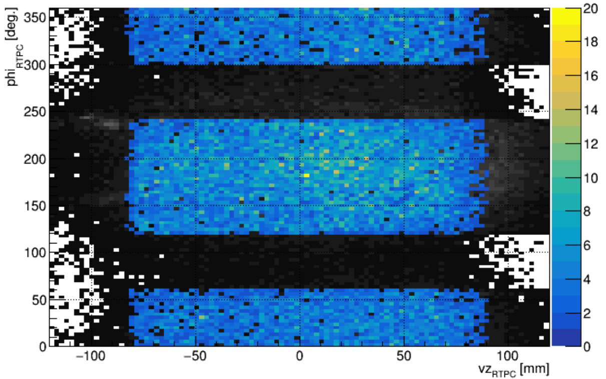
Figure 7.6: RTPC Fiducial Cuts: Distributions of the RTPC hits that fail the cuts are grayscale and the hits that pass are in color.
