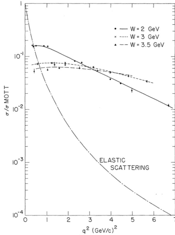
Figure 2.1: DIS: Reduced cross-section as a function of Q^2 [13].
