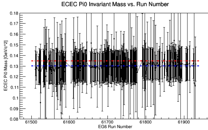
Figure B.7: Invariant mass distribution vs run number zoomed in.
