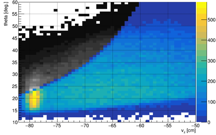
Figure 5.4: Solenoid Fiducial Cut: Particles that have hit the solenoid are rejected.
