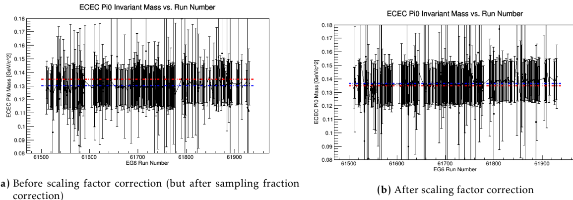
Figure B.16: Comparison of the invariant mass distribution vs run number before (B.16a) and after (B.16b) the scaling factor correction.
