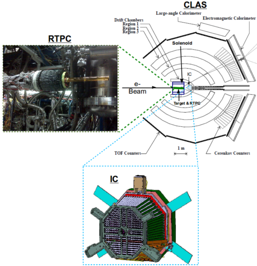
Figure 4.1: The defining upgrades to the CLAS EG6 experiment [3]
