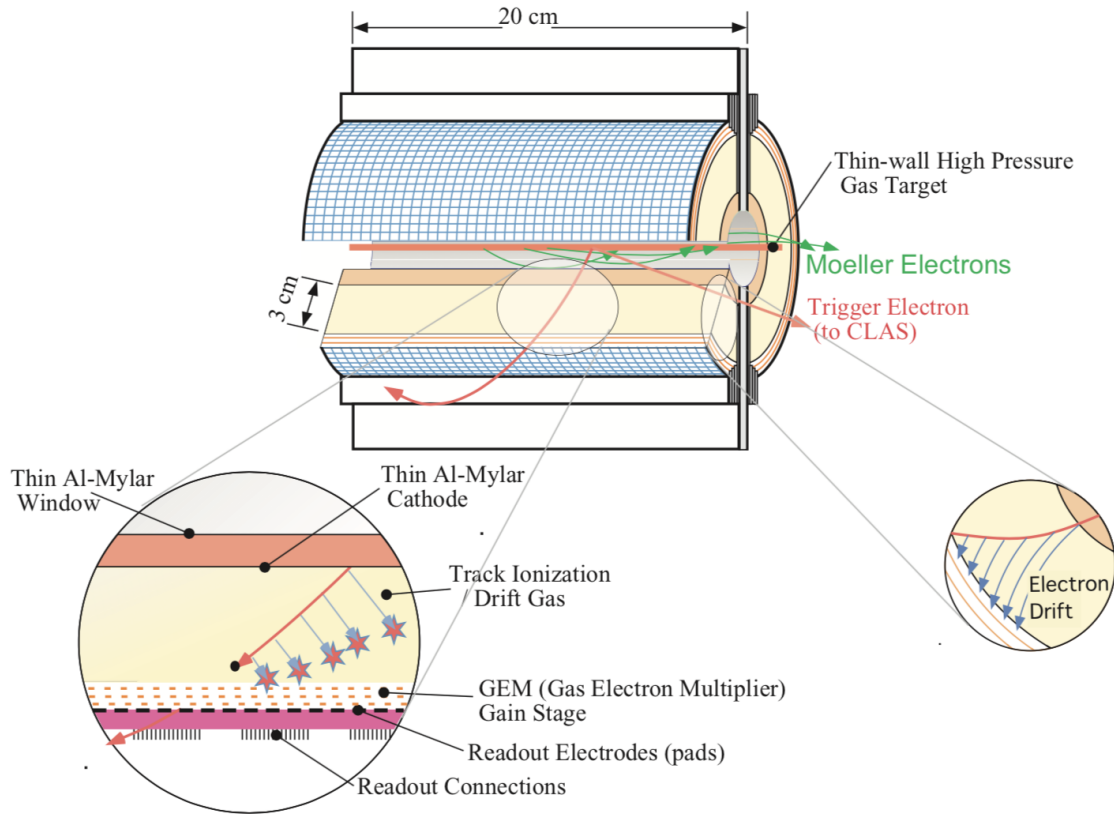
Figure 4.7: The RTPC schematic [1]
