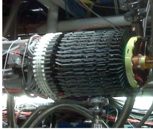
Figure 4.6: The physical RTPC where the beam would be coming from the left [3].
