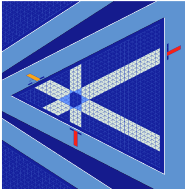
(b) Sector view of EC hit where position is determined from successive hits of the alternating layers scintillation strips
