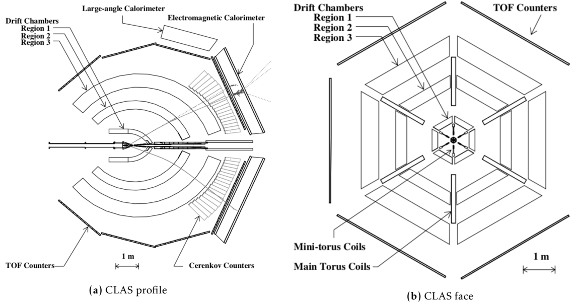
Figure 3.2: Schematic view of CLAS [23]
