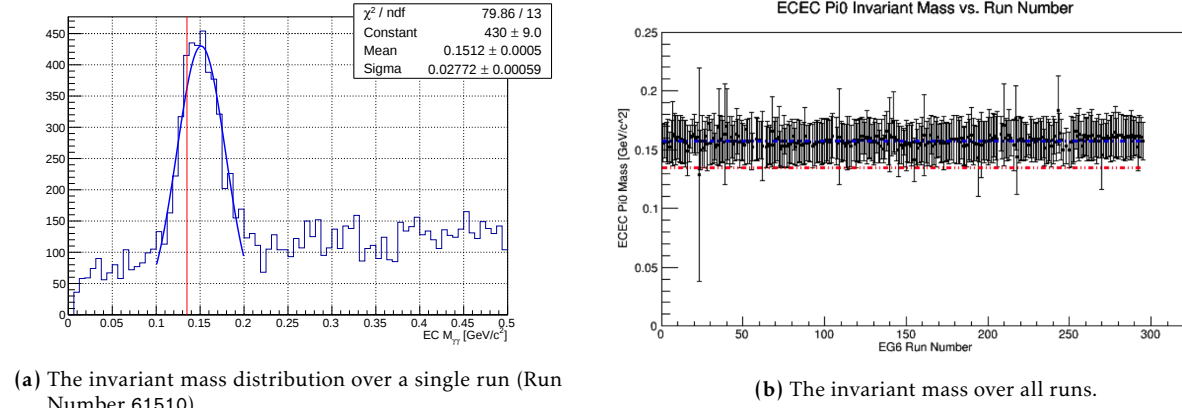
Figure B.3: The invariant mass distribution of EC photon pairs over one run (B.3a) and all runs (B.3b). The red line represents the nominal \pi^0 mass and the blue represents the mean from fit to the data.
