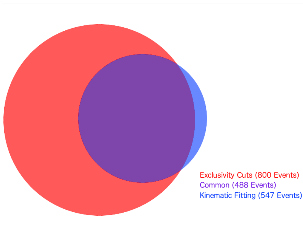
Figure 15.1: Venn diagram of events passing: - Exclusivity cuts (red) - Kinematic fitting with CLC: 0.05 (blue)
