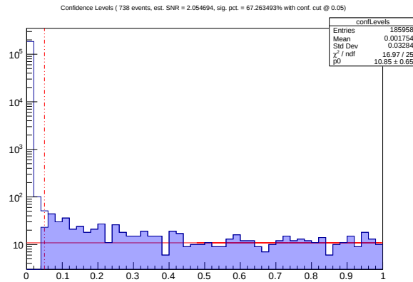
Figure 13.1: Confidence level distribution with a cut at 0.05, represented by the red vertical dashed line. The events passing the cut are represented by the blue highlighted distribution which the right half is fitted to straight line to estimate the signal to noise ratio.
