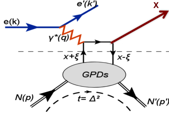
Figure 2.3: “Hand-bag” schematic of deep scattering process where the electron emits a virtual photon that interacts with a parton, producing a particle X before being reabsorbed into the nucleus [3]
