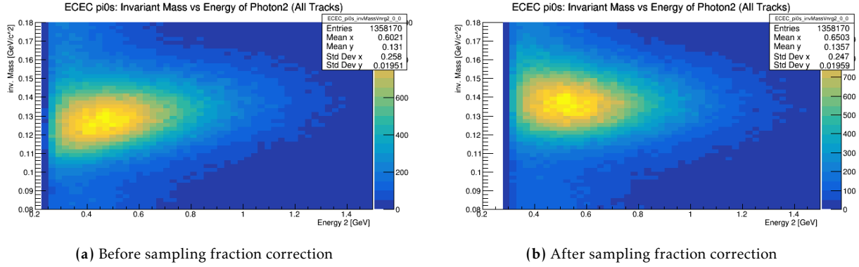
Figure B.15: Comparison of the invariant mass distribution vs energy of lower energy photon before (B.15a) and after (B.15b) the sampling fraction correction.
