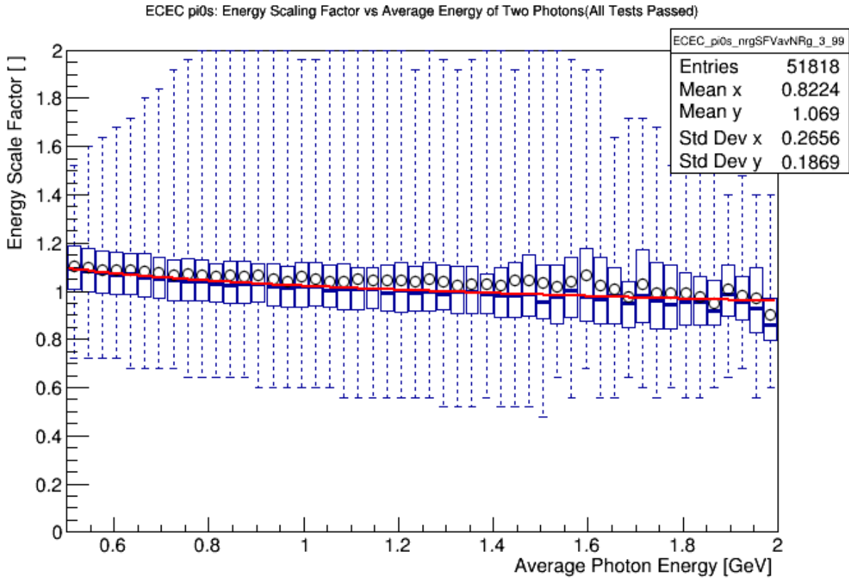
Figure B.12: Scaling factor vs. average energy: Candle-plot profile of Fig. B.10 with fit Eq. B.3.2.4 .
