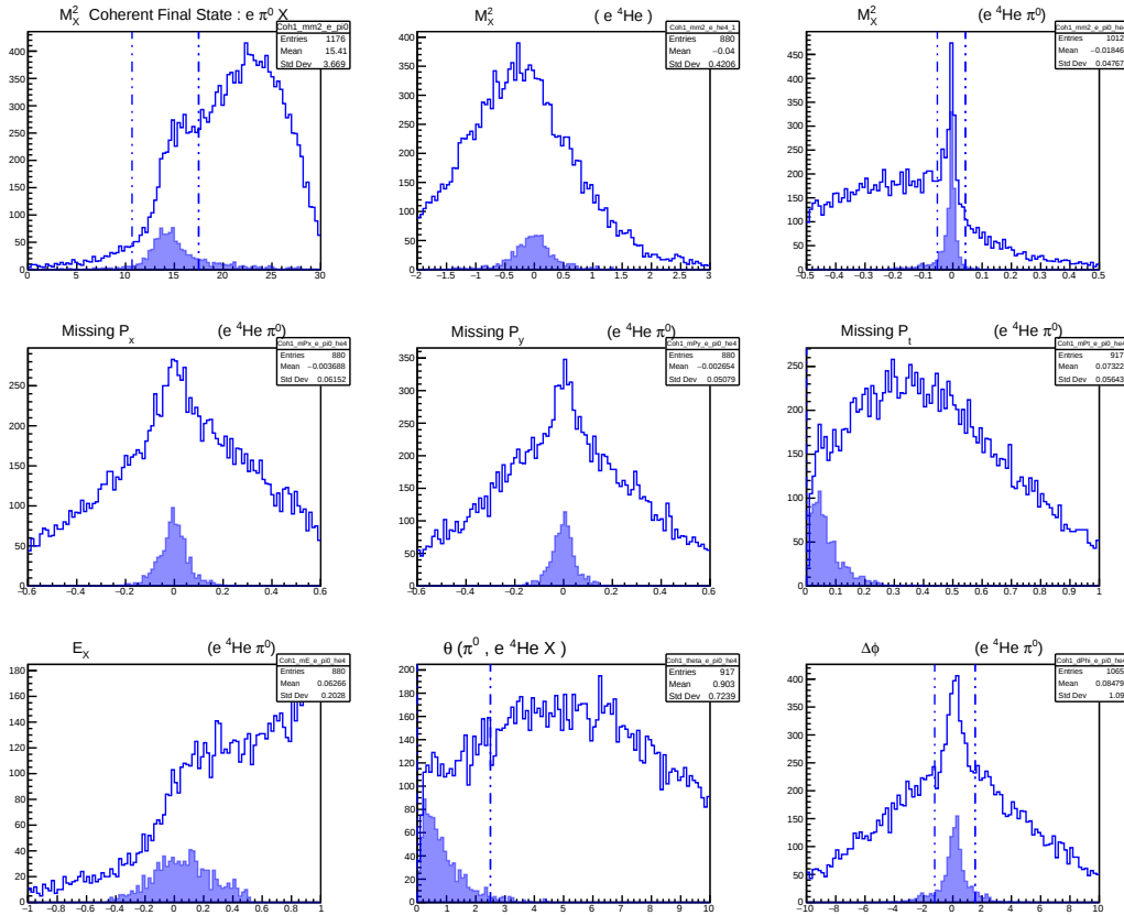
Figure 9.1: Exclusivity cuts on 4 variables shown with dashed vertical lines. The events passing all other cuts except for its own cut are highlighted in light blue. All other events detecting an electron, helium-4, and two photons is the unshaded histogram.
