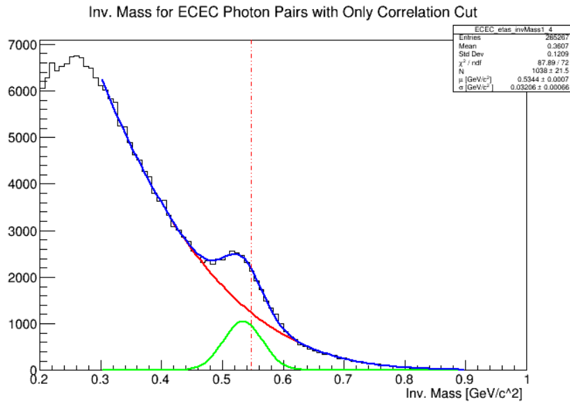
Figure B.18: Invariant mass distribution EC photons coming from neighboring sectors. The blue, red, and green are the full corrected, fitted background, and the extracted signal (from subtracting fitted background distribution from full distribution) distributions, respectively. The red is the nominal value of the \eta invariant mass.
