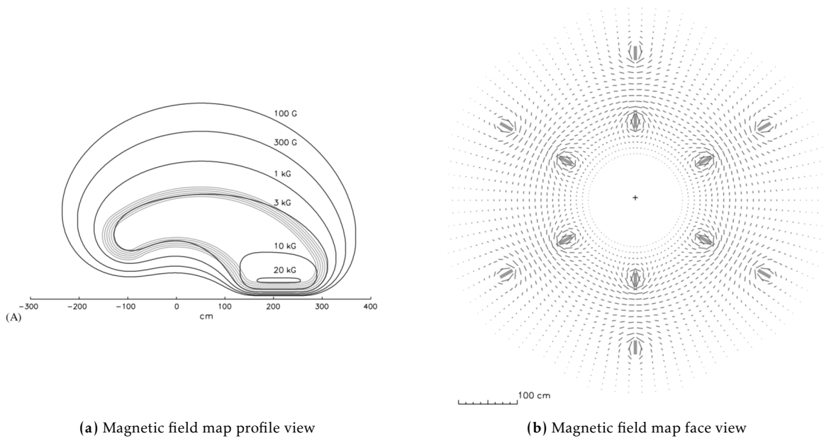
Figure 3.3: Torus magnet's field maps [23]
