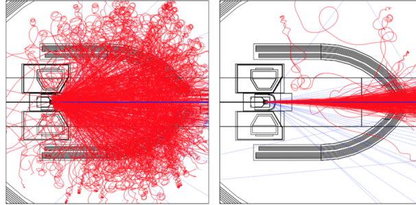
Figure 4.4: Affect of solenoid \vec{B} -field: GEANT simulation of the Møller electrons, in red, with (right) and without (left) the solenoid field [3].
