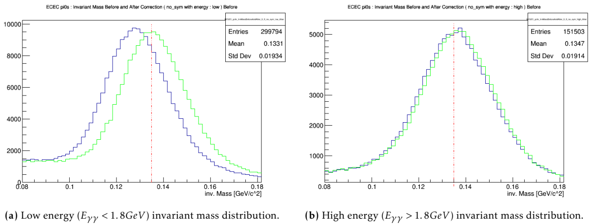
Figure B.14: Invariant mass distribution for low (B.14a) and high (B.14b) energy generic EC \pi^0 . The blue and green are the uncorrected and corrected distributions, respectively. The red is the nominal value of the \pi^0 invariant mass.
