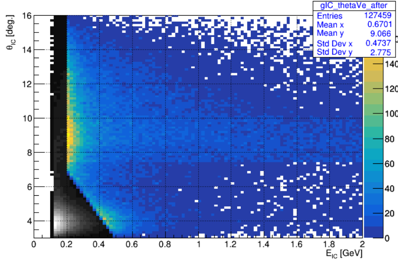
Figure 6.5: Møller Electron Cut: A geometric cut is applied to reject low-energy, low-angle Møller electrons
