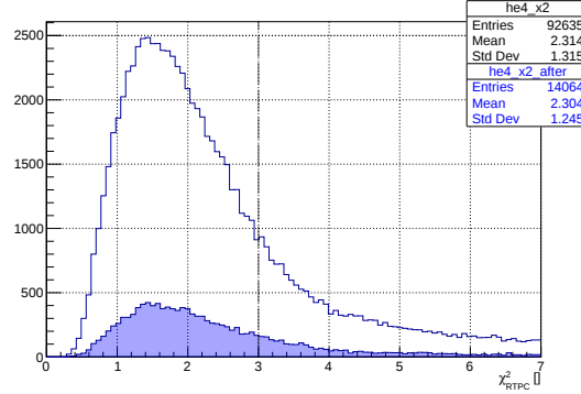
Figure 7.2: \chi^2 Cut: The \chi^2 -distribution obtained from fitting the RTPC tracks correspond to how well the ionization points are fit. High \chi^2 , corresponding to poor fits, are rejected.
