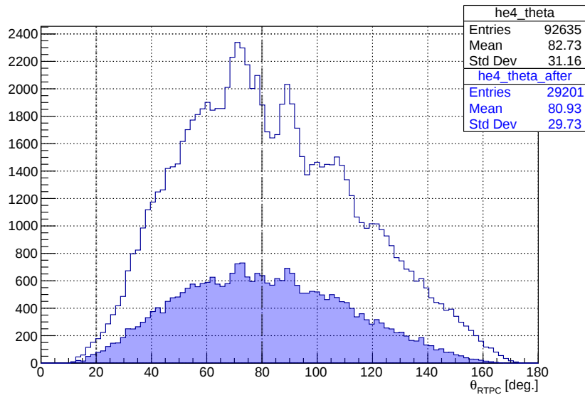
Figure 7.4: \theta Cut: Backward traveling tracks are rejected.
