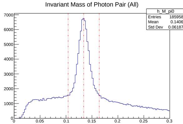
Figure 9.2: The invariant mass distribution of two photons in the IC. The central vertical dashed line is the nominal value and the ones to the left and right are the \pm 3\sigma cut values.
