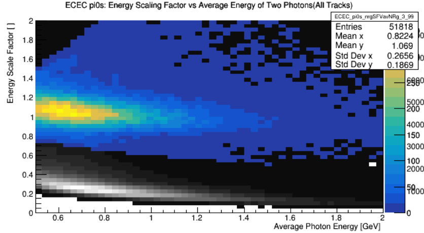
Figure B.10: Scaling factor vs. average energy: The energy scaling factor decreases with increasing energy.
