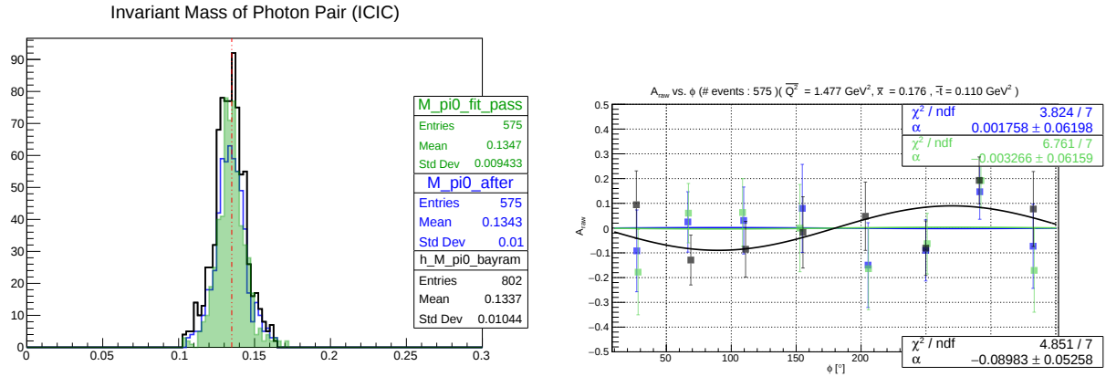
(a) Invariant mass distributions of photon pairs with the nominal value indicated by the vertical red line (b) Raw beam spin asymmetries integrated over all Q^2, x, -t bins
