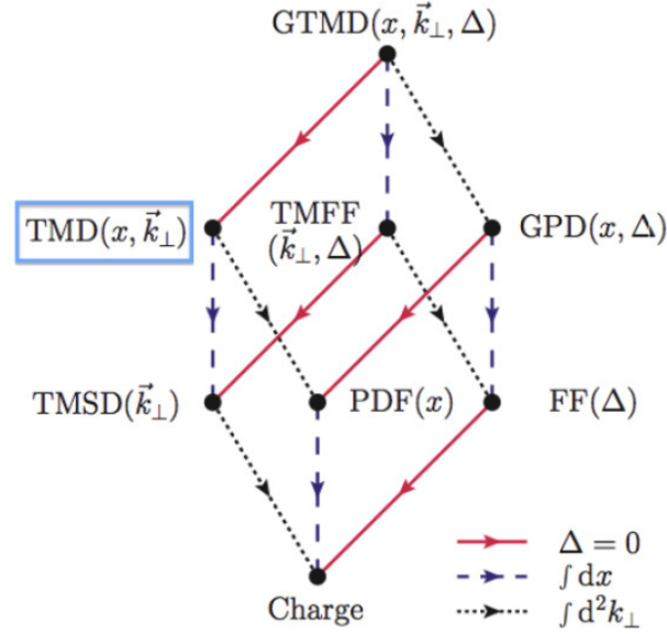
Figure 2.2: Schematic of GTMD and its reduction to different measurable quantities: structure functions [3].
