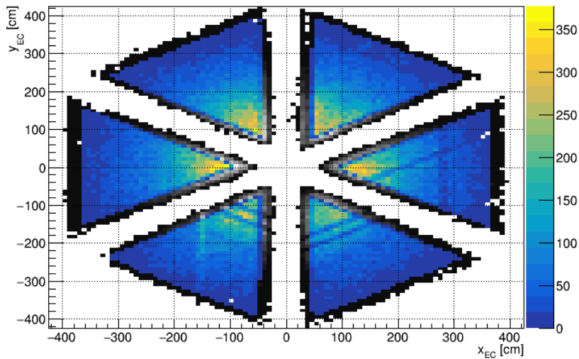
Figure 5.9: EC Fid Cut: x- and y-coordinates of the face of the EC that are rejected (grayscale) and accepted (colored).
