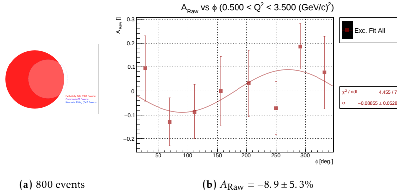
Figure 15.3: Beam spin asymmetry (b) of selected events (a): All events passing exclusivity cuts
