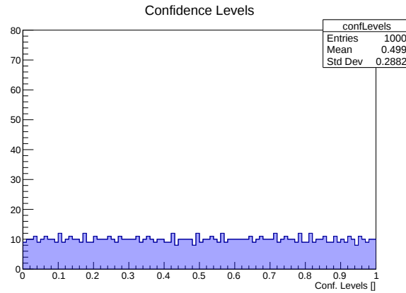
Figure 10.1: Sample of confidence level distribution with no background. Events selected are highlighted in blue.
