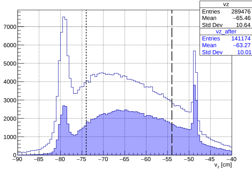
Figure 5.3: Vertex Cut: Only particles coming from well inside the target walls are accepted.
