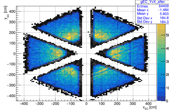
Figure 6.3: EC Fid. Cut: Reject particles hitting the edges of the EC.
