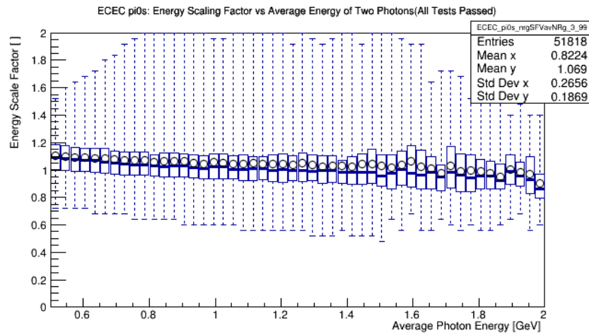
Figure B.11: Scaling factor vs. average energy: Candle-plot profile of Fig. B.10 .
