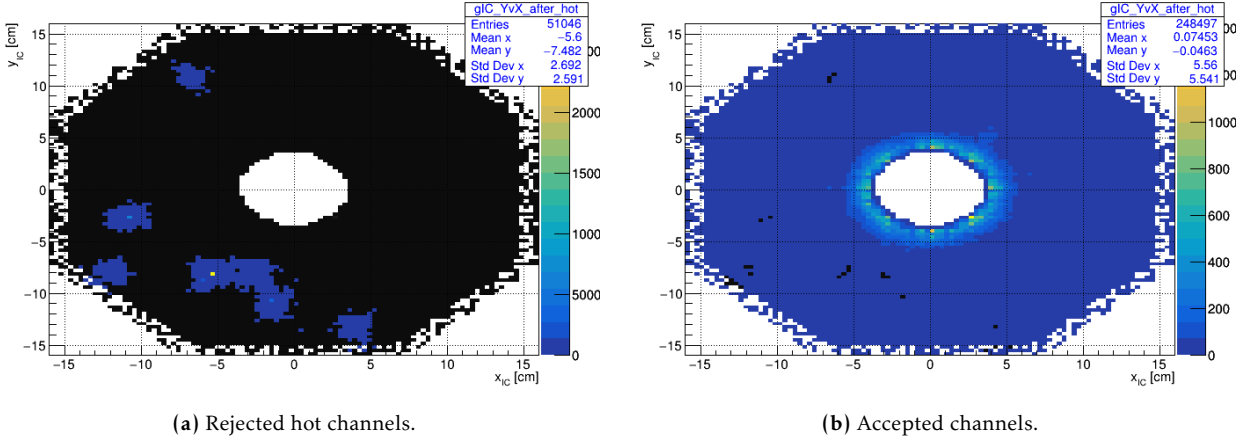
Figure 6.6: Hot Channels Cut: The position of the hits in the IC that are rejected (6.6a) and accepted (6.6b) by the cut.
