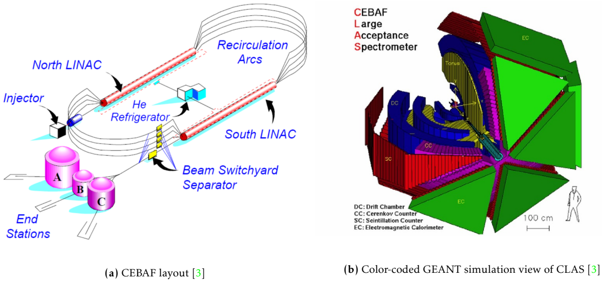
Figure 3.1: CEBAF (a) and CLAS (b) [3]
