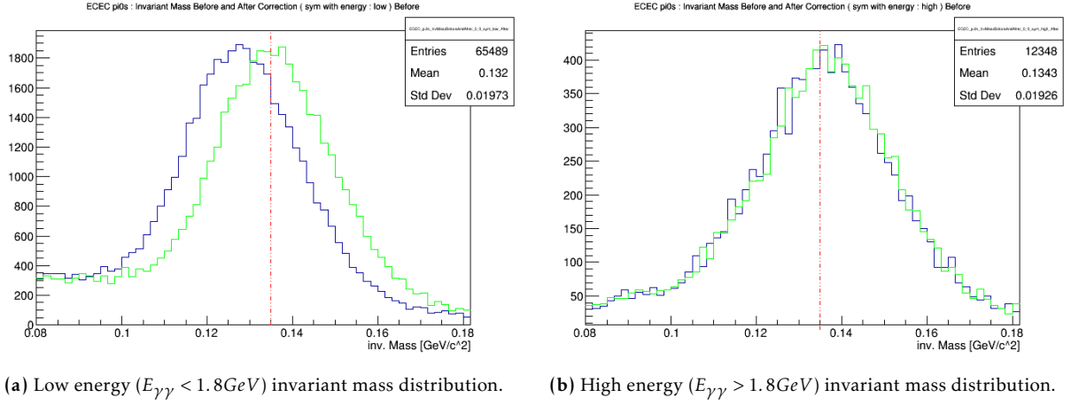
Figure B.13: Invariant mass distribution for low (B.13a) and high (B.13b) energy symmetric EC \pi^0 . The blue and green are the uncorrected and corrected distributions, respectively. The red is the nominal value of the \pi^0 invariant mass.
