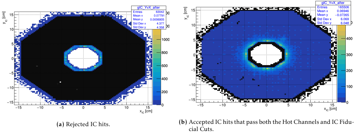
Figure 6.7: IC Fiducial Cut: The position of the hits in the IC that are rejected (6.7a) by the cut and accepted (6.7b) by both the Hot Channels and Fiducial Cuts (to see features).
