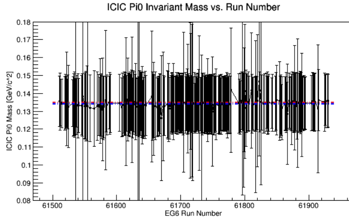
Figure B.8: Invariant mass distribution vs run number of IC photons.
