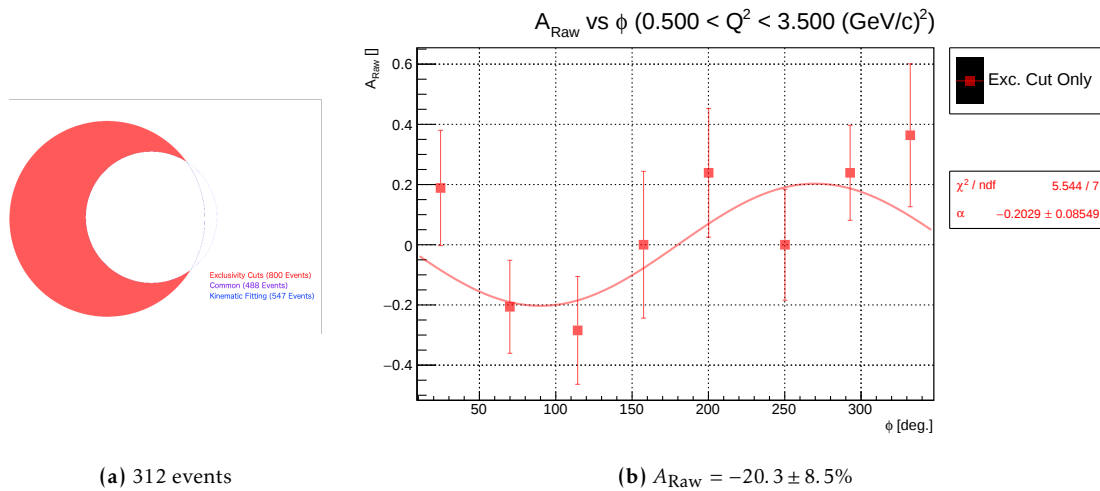
Figure 15.6: Beam spin asymmetry (b) of selected events (a): Events passing only exclusivity cuts
