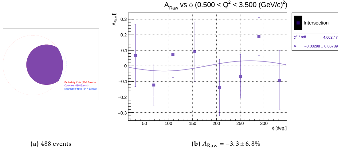
Figure 15.5: Beam spin asymmetry (b) of selected events (a): Events passing both exclusivity cuts and kinematic fitting
