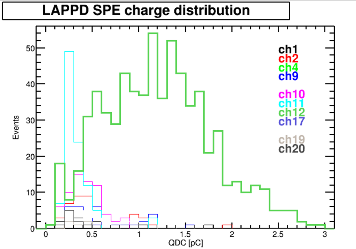
Figure 7: Charge distribution of single photoelectron signal at a mean gain of about 7 \times 10^6 .
