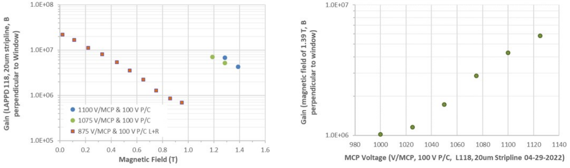
Figure 2: LAPPD 118 test results in magnetic field: (left) Gain decreased with increasing magnetic field; (right) Gain recovered with a higher MCP voltage.
