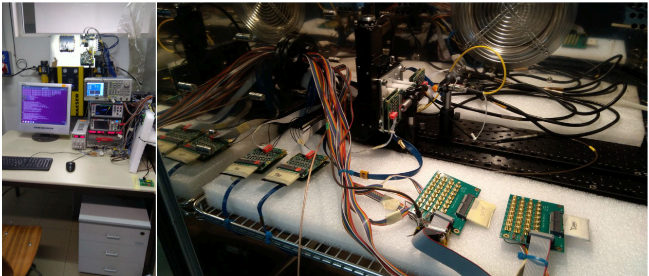
Figure 11: Control, HV and readout electronics (left) and SiPM sensor cards in the climatic chamber (right) in the SiPM Bologna characterization setup. The motor stage with the LED is also visible.
