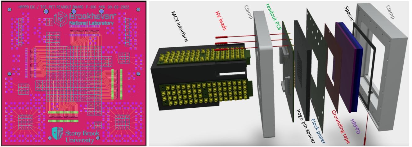
Figure 10: Left: a compact multi-pattern dual purpose readout board, to be used for both EIC-related HRPPD / LAPPD evaluation and in a joint SBU / BNL Time of Flight Positron Emission Tomography project. It will be instrumented with pogo pins and connectors in several different configurations. Right: an expanded view of the HRPPD enclosure, with a readout PCB shown in a configuration with a central 16x16 pixel field instrumented.
