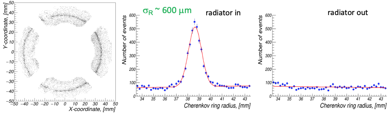
Figure 4: Cherenkov ring radius resolution in a configuration with a 120 GeV proton beam passing through a 14 mm thick aspheric lens radiator with effective focal length of 20 mm. Left: detected single photon cluster positions exhibit a sharp circular pattern with the expected diameter of \sim 76 mm. Center: radial width of this circular pattern defines the upper limit of the achievable spatial resolution for a given signal-to-noise ratio (raw spectrum, none of the instrumental effects unfolded). Right: background spectrum, with the lens radiator taken out of the beam.
