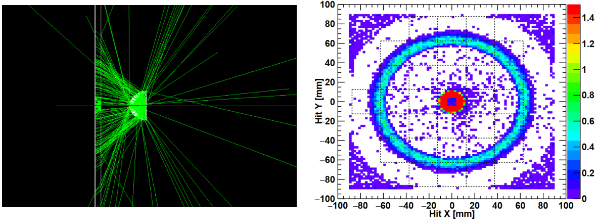
Figure 9: Left: Monte Carlo study of the Cherenkov light generated in the lens-shaped quartz radiator, side view. Right: Image of the hits detected in the LAPPD by the Cherenkov light generated in the lens-shaped quartz radiator.
