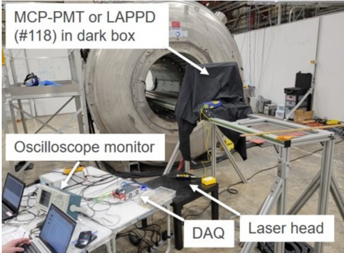
Figure 1: Experiment setup for magnetic field test at ANL.
