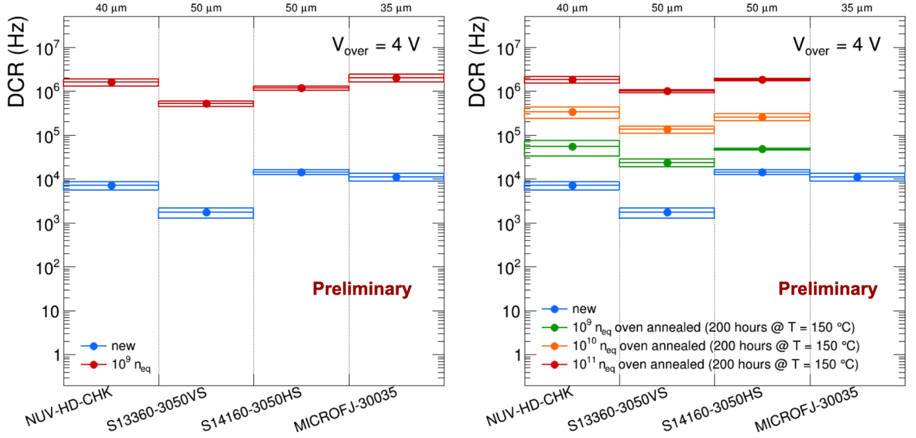
Figure 12: DCR values measured on sensors from Hamamatsu, FBK and OnSemi after irradiation (left), and recovery after annealing in oven.
