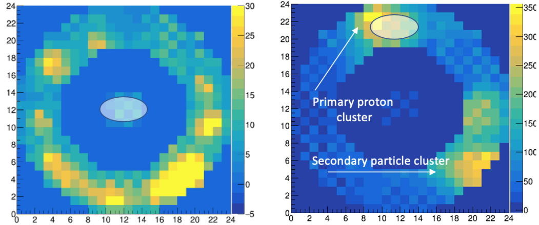
Figure 5: Typical single events as detected by LAPPD 136 equipped with a readout board shown in figure 3. Intensity scale is given in [mV]. Beam spot is indicated by a grey oval. Left: configuration with the aspheric lens radiator and beam passing through the center of the circular pad pattern. Several single photon clusters with amplitudes up to few dozens of mV are seen in the top half of the pad pattern. The bottom half is flooded by photons, indicating that the lens was hit by a beam proton close to its top left side. Right: configuration with the beam centered at the top side of the pad area itself, and LAPPD quartz window used as a radiator. A high energy hadron produces dozens of Cherenkov photons in a 5mm thick UV-grade quartz window, generating pulses of several hundred mV. A small fraction of events contains additional clusters generated by secondary particles originated in the upstream target (bottom right side of the pad pattern in this particular event). Relative timing resolution between such pairs of clusters in the same event can be used as a measure of a possible Time-of-Flight LAPPD performance in the ePIC detector electron-going endcap where secondary particles pass through the sensor window.
