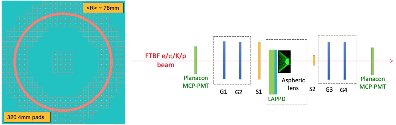
Figure 3: Left: one of the quadrants of the readout board designed for the Fermilab beam test in June 2022. Right: schematics of the beam test setup, shown in a configuration with the aspheric lens radiator (S1..S2 - scintillation counters, G1..G4 - GEM tracker stations).
