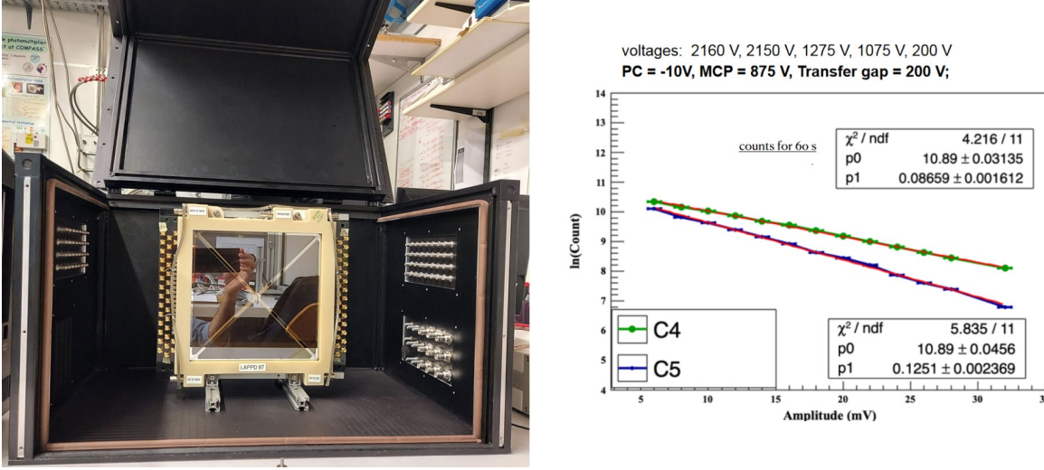
Figure 6: Left: The dark box used for the LAPPD studies at INFN. Right: Example of dark rate measurements: rates versus threshold.
