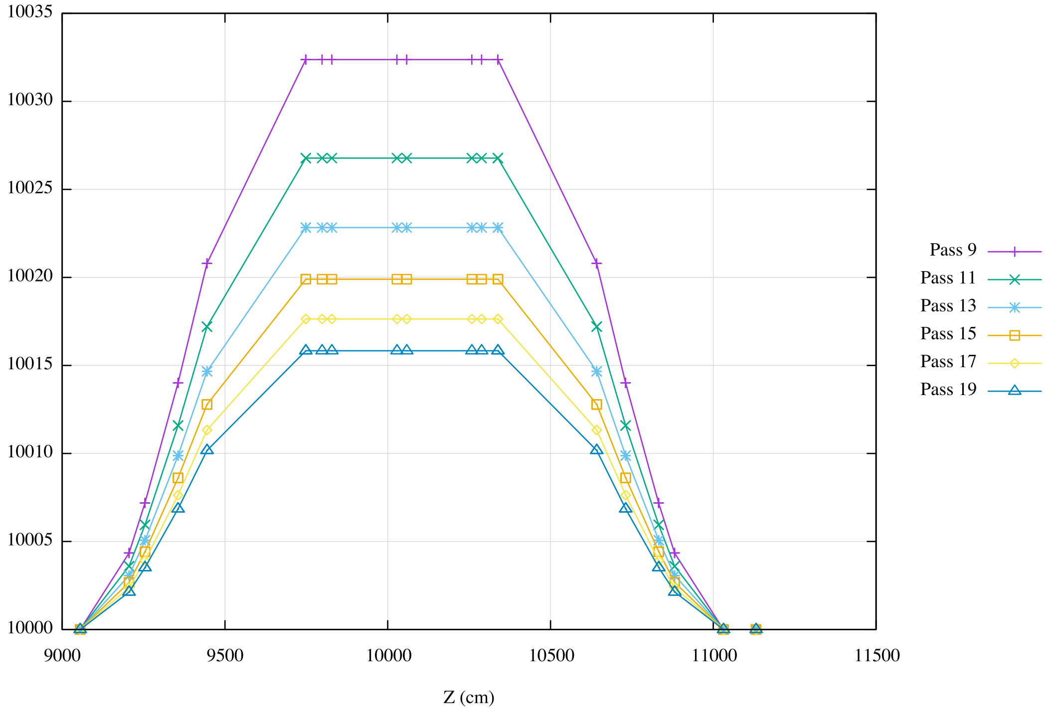
Vertical Orbit Spread in FFA Branch of NE Spreader vs. Z
