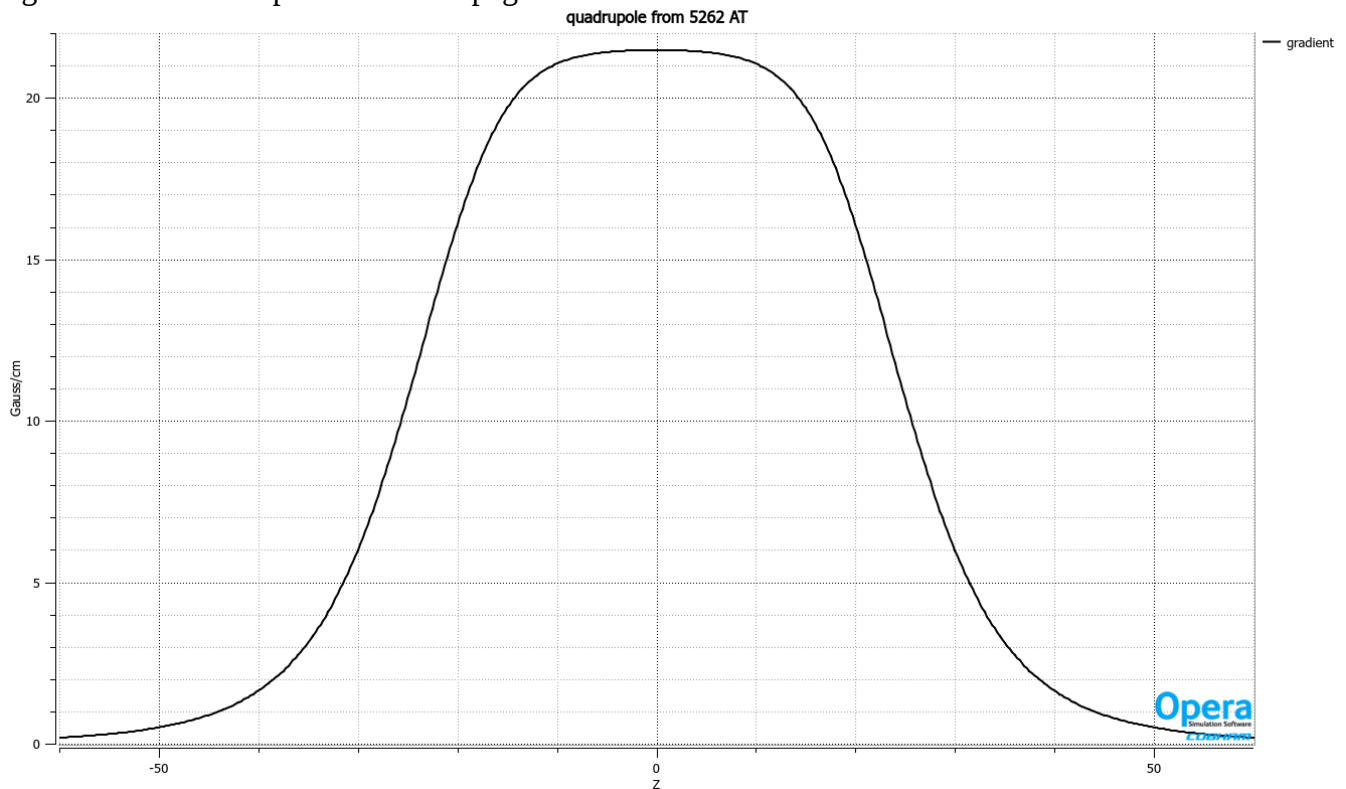
Figure 4. Gradient provided by the quadrupole coil at 5262 AT. Peak is 215 mT/m, 1.2x the request of 3 \times 60 mT/m on page one.
