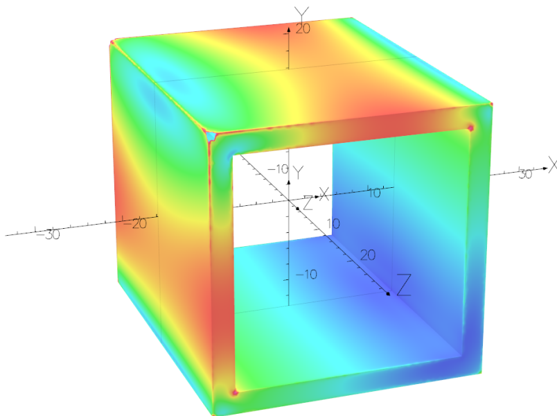
Figure 2. Field on the surface of the steel with 6578 AT in quad coils and 6420 AT in dipole coils. Resulting fields exceed the requirements on page one. It is unlikely that all coils will be energized at once, much less at maximum, but the steel should be sized to allow this. It is expected that only one of the dipoles will be powered in each unit, corresponding to the type of gradient provided in the permanent magnet: horizontal correction for focusing, vertical correction for defocusing.
