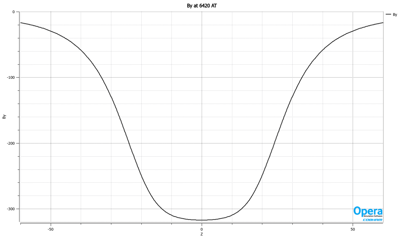
Figure 3. B_y(z) for the dipole which moves beam horizontally. Just under 320 G is available, in agreement with the specification on page one.
