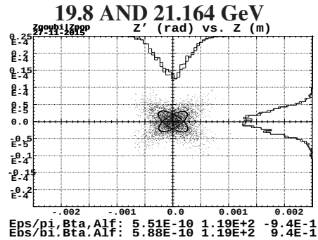
Figure 30: Bunch transverse emittances (non normalized) and \beta_x , \alpha_x , \beta_y , \alpha_y parameters are given at the bottom of the plot for each energy. These parameters appear to be well preserved, with \beta_y betatron damping as expected ( i.e. , same normalized emittances at linac entrance and exit).
