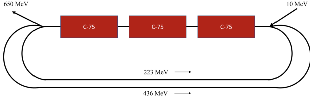
Figure 2: A conceptual layout of the new 650 MeV injector.
