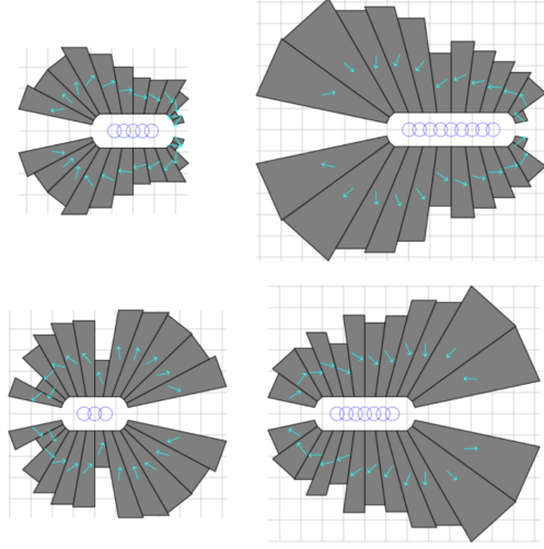
Figure 4: Focusing (top) and defocusing (bottom) 2D permanent magnet designs for the FFA arcs. The left column is a design including sextupole components while minimizing magnet volume. The right column is the baseline design.
