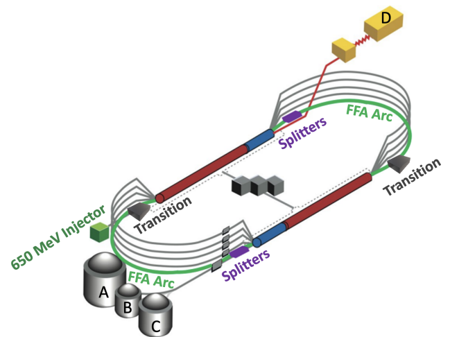
Figure 1: The current 22 GeV CEBAF baseline design. It consists of the upgraded 650 MeV injector (green box), linacs (red and blue), EM arcs (grey curves), FFA arcs (green curves), Splitters (purple), Transition (dark grey), and four experimental halls (A – D).
