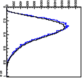
Buranol (black) and CH2 (blue) pt_p
