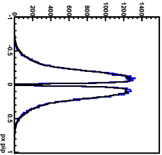
Buranol (black) and CH2 (blue) px_pip
