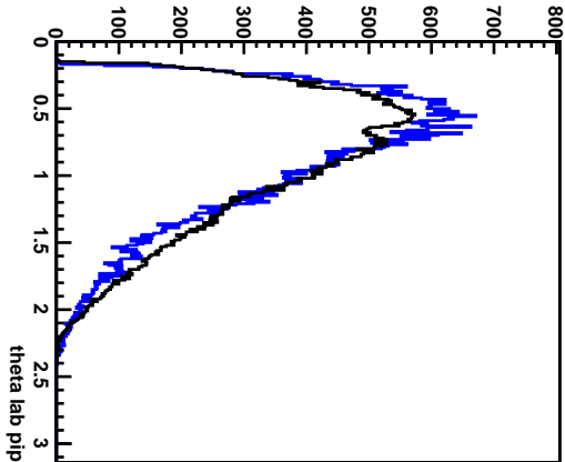
Butanol (black) and CH2 (blue) theta_lab_pip
