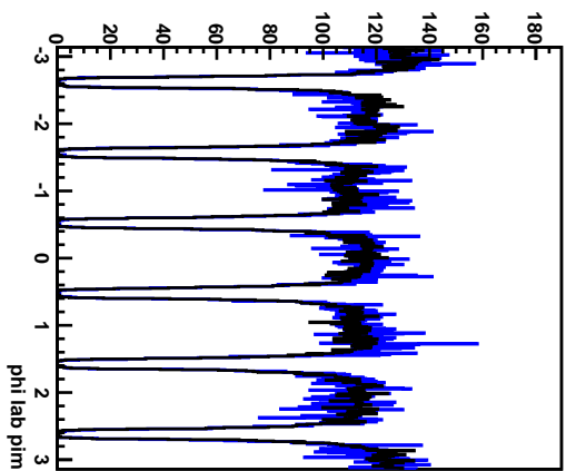
Butanol (black) and CH2 (blue) phi_lab_pim
