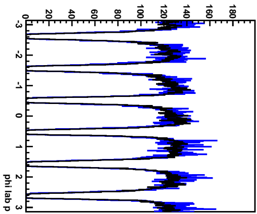
Butanol (black) and CH2 (blue) phi_lab_p
