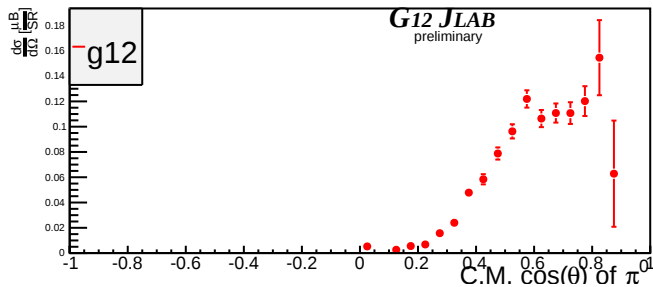
Beam Energy 3.475 GeV \pm 25MeV
