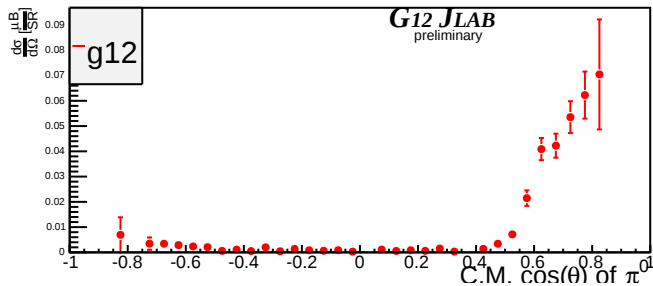
Beam Energy 5.075 GeV \pm 25MeV
