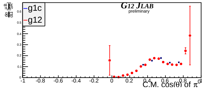
Beam Energy 2.925 GeV \pm 25MeV
