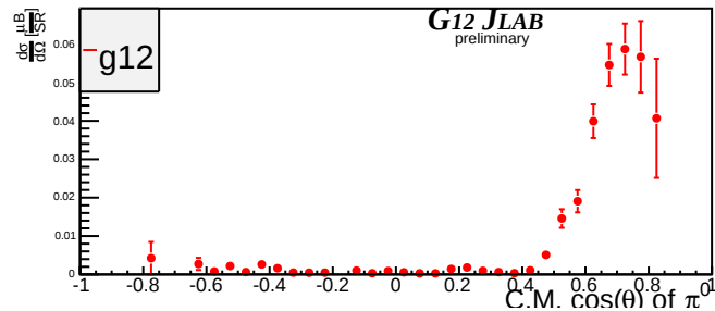
Beam Energy 5.125 GeV \pm 25MeV
