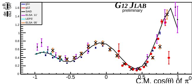
Beam Energy 1.775 GeV \pm 25MeV
