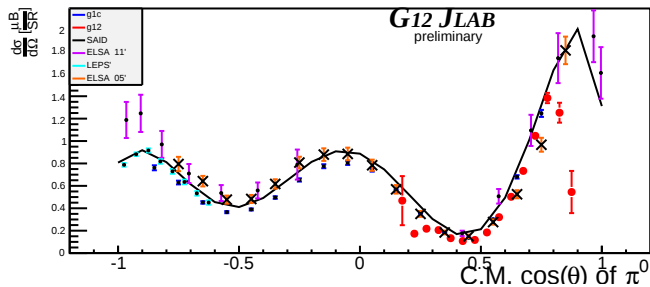
Beam Energy 1.675 GeV \pm 25MeV
