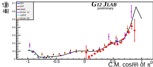
Beam Energy 2.375 GeV \pm 25MeV
