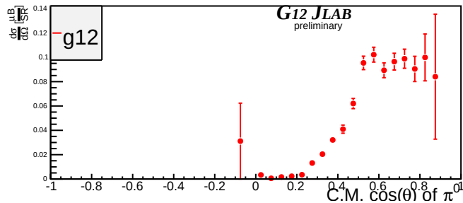
Beam Energy 3.525 GeV \pm 25MeV
