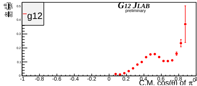
Beam Energy 3.025 GeV \pm 25MeV
