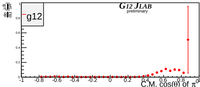
Beam Energy 3.875 GeV \pm 25MeV
