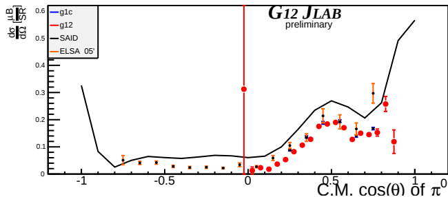
Beam Energy 2.675 GeV \pm 25MeV
