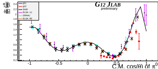
Beam Energy 1.525 GeV \pm 25MeV
