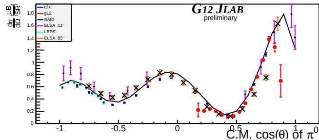
Beam Energy 1.725 GeV \pm 25MeV
