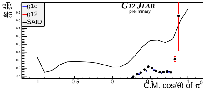
Beam Energy 2.875 GeV \pm 25MeV
