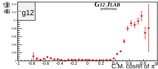
Beam Energy 4.125 GeV \pm 25MeV
