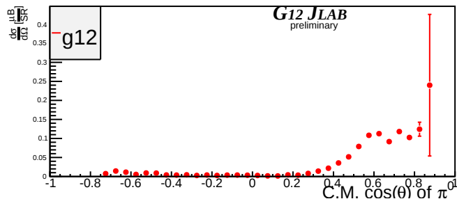
Beam Energy 3.625 GeV \pm 25MeV
