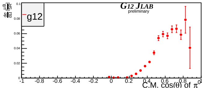
Beam Energy 3.575 GeV \pm 25MeV
