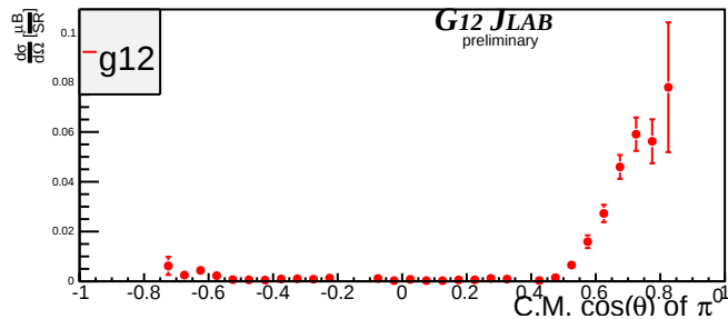
Beam Energy 5.325 GeV \pm 25MeV
