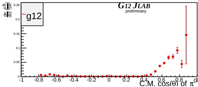
Beam Energy 4.675 GeV \pm 25MeV
