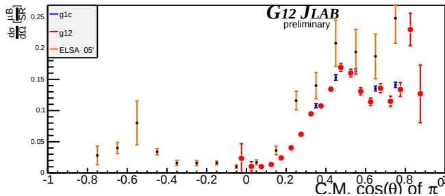
Beam Energy 2.975 GeV \pm 25MeV
