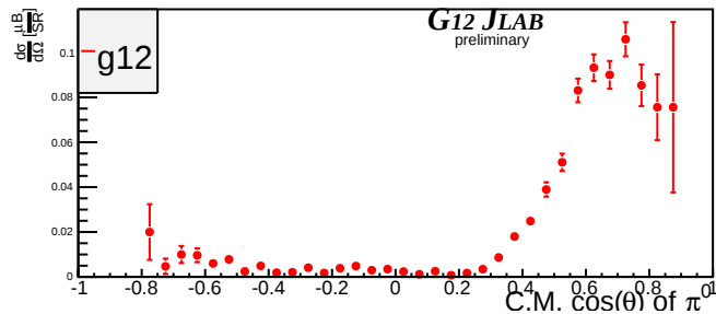
Beam Energy 3.825 GeV \pm 25MeV
