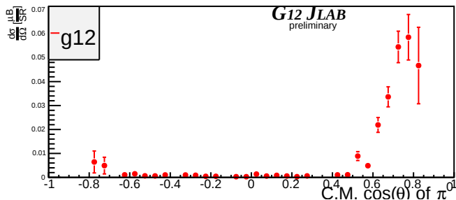
Beam Energy 5.375 GeV \pm 25MeV
