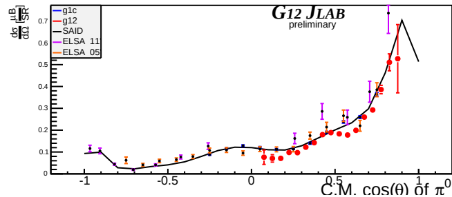
Beam Energy 2.425 GeV \pm 25MeV
