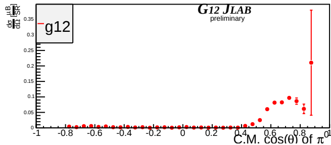
Beam Energy 4.425 GeV \pm 25MeV
