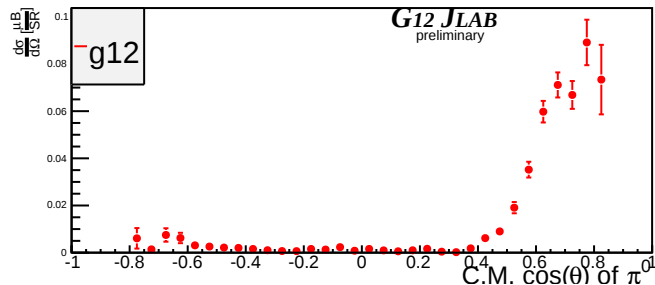
Beam Energy 4.525 GeV \pm 25MeV
