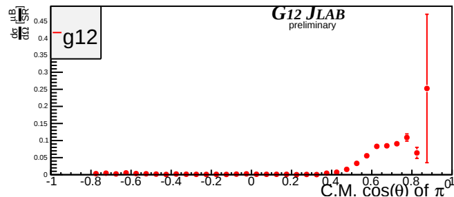
Beam Energy 4.225 GeV \pm 25MeV
