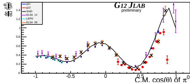
Beam Energy 1.825 GeV \pm 25MeV
