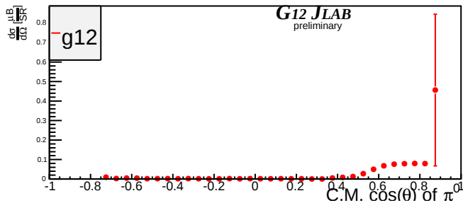
Beam Energy 4.375 GeV \pm 25MeV
