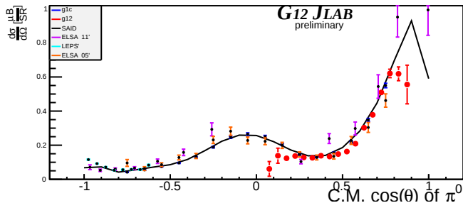
Beam Energy 2.075 GeV \pm 25MeV
