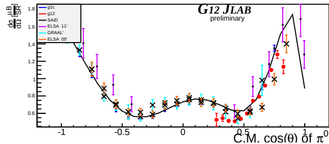
Beam Energy 1.425 GeV \pm 25MeV
