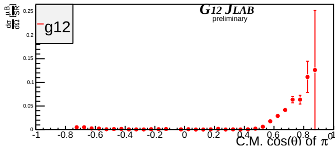
Beam Energy 5.275 GeV \pm 25MeV
