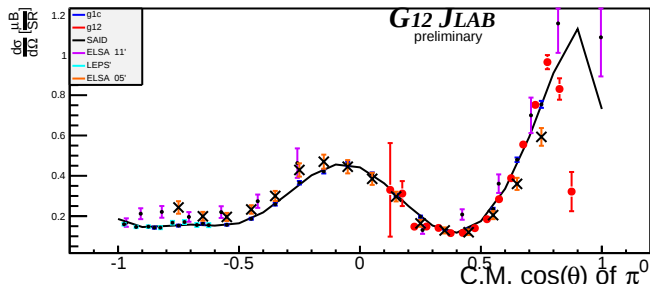
Beam Energy 1.975 GeV \pm 25MeV
