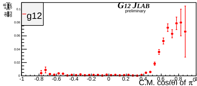
Beam Energy 4.725 GeV \pm 25MeV
