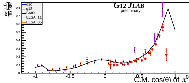
Beam Energy 2.325 GeV \pm 25MeV
