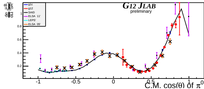
Beam Energy 2.025 GeV \pm 25MeV
