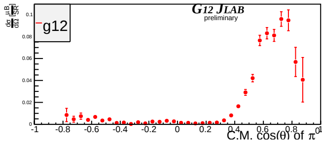
Beam Energy 4.075 GeV \pm 25MeV
