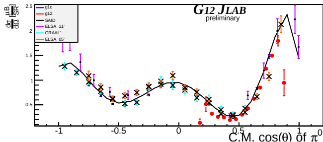
Beam Energy 1.475 GeV \pm 25MeV
