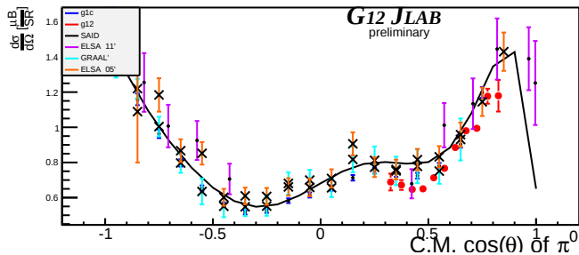
Beam Energy 1.375 GeV \pm 25MeV
