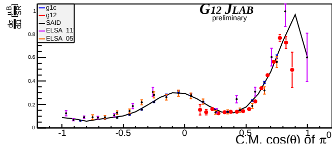
Beam Energy 2.125 GeV \pm 25MeV
