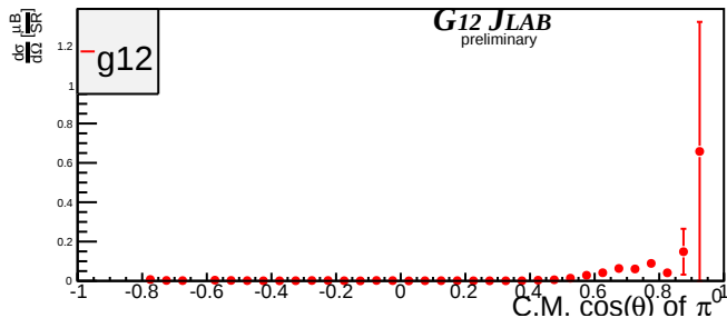
Beam Energy 4.775 GeV \pm 25MeV
