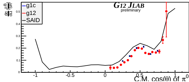
Beam Energy 2.725 GeV \pm 25MeV
