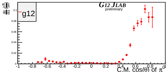
Beam Energy 4.175 GeV \pm 25MeV
