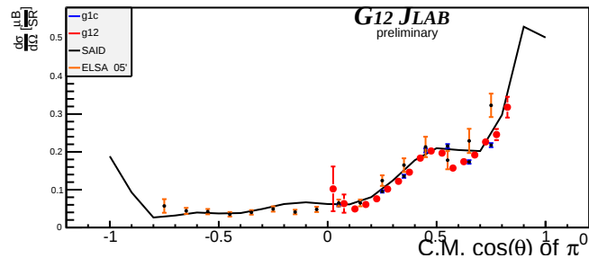
Beam Energy 2.625 GeV \pm 25MeV
