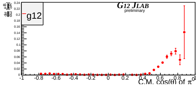
Beam Energy 4.825 GeV \pm 25MeV
