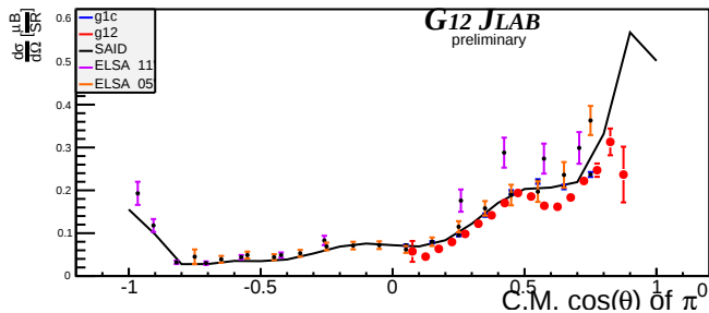
Beam Energy 2.575 GeV \pm 25MeV
