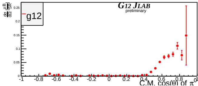
Beam Energy 4.475 GeV \pm 25MeV
