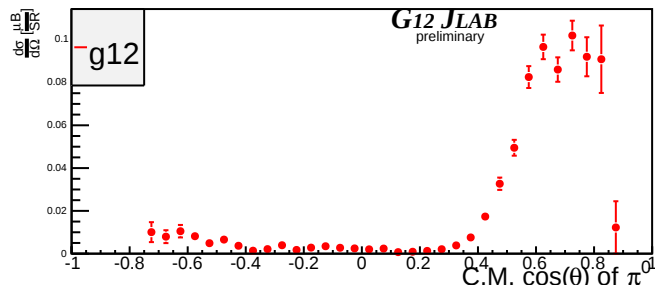
Beam Energy 3.925 GeV \pm 25MeV
