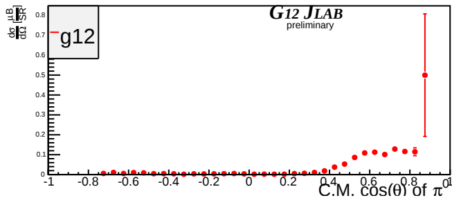
Beam Energy 3.775 GeV \pm 25MeV
