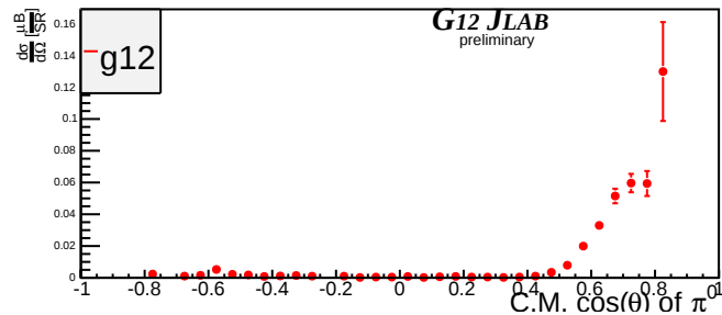
Beam Energy 5.025 GeV \pm 25MeV
