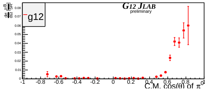
Beam Energy 5.425 GeV \pm 25MeV
