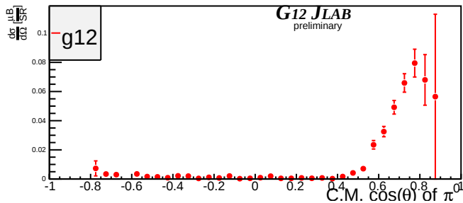
Beam Energy 4.975 GeV \pm 25MeV
