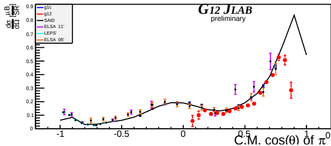
Beam Energy 2.275 GeV \pm 25MeV
