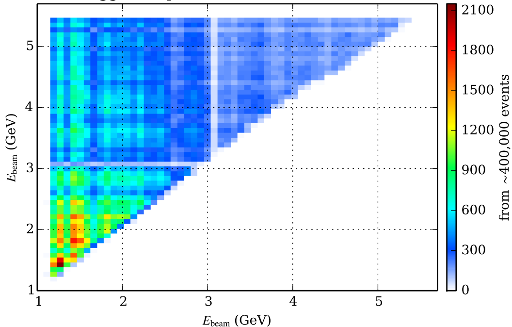
All tagger-hit pairs within 1 ns (RF corrected)
