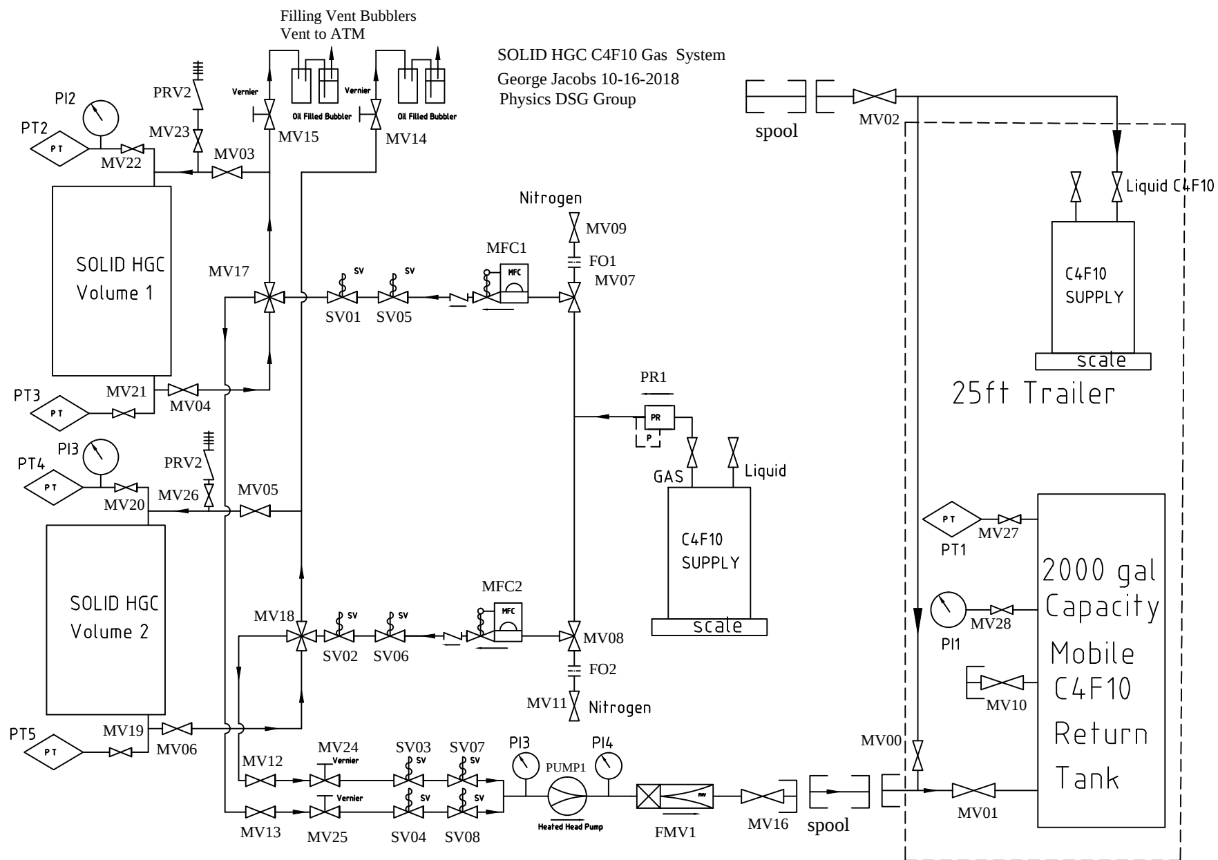
Hall A SOLID Heavy Gas Cerenkov C4F10 Gas System P&I
