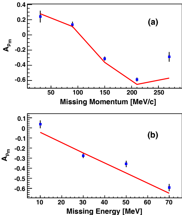
FIG. 13. The measured missing momentum asymmetry as a function of the missing momentum (a) and missing energy (b) for Q^2=8.0(\text{GeV}/c)^2 . The red line indicates the simulated values for the corresponding points.
