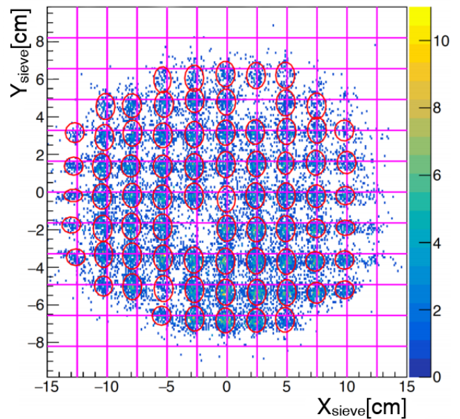
FIG. 2. Reconstructed sieve aperture pattern for the central target foil in the SHMS. The central hole is half diameter compared to the other sieve holes (6 mm diameter), and two empty sieve positions are observed to be consistent with sieve holes that are blocked.
