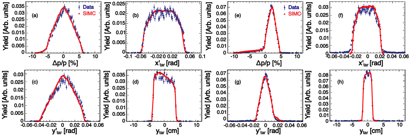
FIG. 3. The reconstructed angles at the target and momentum for data (blue) and simulated spectra (red) for the measured H(e, e'p) reaction with arbitrary normalization. Panels (a) - (d) show the momentum bite \Delta p/p (a), vertical angle ( x'_{tar} ) (b), horizontal angle ( y'_{tar} ) (c) and reconstructed horizontal position ( y_{tar} ) for the electrons in the HMS. Panels (e) - (g) show the momentum bite \Delta p/p (e), vertical angle (f), horizontal angle (g), and reconstructed horizontal position (h) for the proton in the SHMS.
