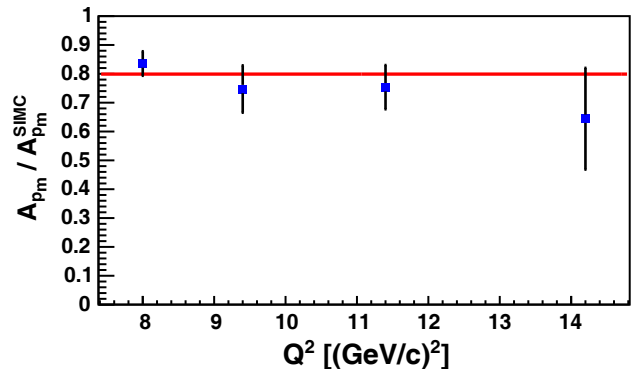
FIG. 14. The ratio of the A_{p_m} asymmetry in data to simulation as a function of Q^2 . The red line is the constant value fit to the data.
