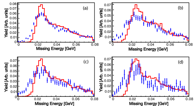
FIG. 7. Carbon missing energy spectra for the experimental data (blue points) for each of the 4 kinematics, (a) 8, (b) 9.4, (c) 11.4, and (d) 14.4 (GeV/c) ^2 compared to simulation for the corresponding kinematics (red line). These spectra include both the 1s_{1/2} and 1p_{3/2} shell contributions.
