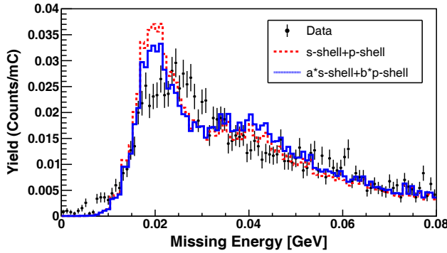
FIG. 9. The dashed red distribution is the sum with unit weights of the 1s_{1/2} shell and 1p_{3/2} contributions, the solid blue distribution is the a(1s_{1/2}) + b(1p_{3/2}) distribution for best fit to the data as described in the text. The black points with error bars are the data (statistical errors only). All the distributions correspond to Q^2 = 8 (\text{GeV}/c)^2 kinematics.
