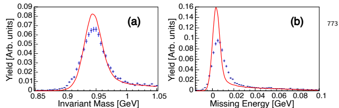
FIG. 6. The comparison between simulation and data (with arbitrary normalization) is shown for the Q^2=8 (GeV/c) ^2 setting. The reconstructed W (a) is primarily driven by the electron arm (HMS) reconstruction, while the missing energy (b) includes contributions from the proton arm (SHMS).
