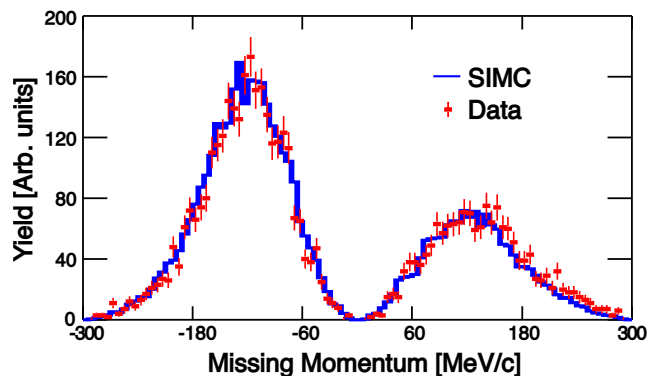
FIG. 12. The missing momentum distribution is shown for the kinematic setting at Q^2 = 8 (GeV/c) 2 where the simulation is normalized to the data.
