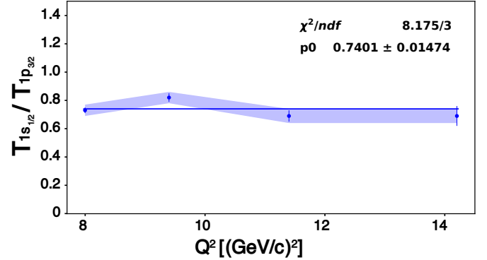
FIG. 11. The ratio of transparencies for the 1s_{1/2} shell to the 1p_{3/2} shell protons as a function of Q^2 . The error bars show the statistical uncertainty, while the band represents the total systematic uncertainty. The solid line shows the fit to a constant value.
