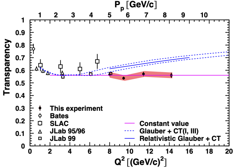
Figure 2: All present carbon electron-scattering results are shown including the latest Hall C measurement [10] indicating no onset in CT up to Q^2 = 14.2 \text{ GeV}^2/c^2 .
