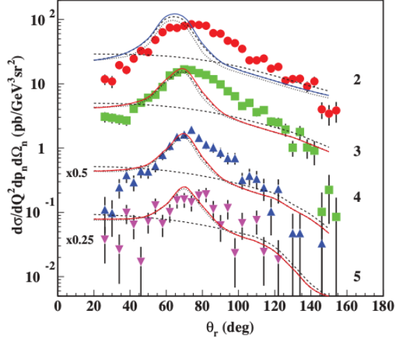
Figure 5: Data from [48] shows the dependence of the differential cross section on the recoil neutron angle and momentum where the momentum of the recoil neutron for these data is restricted to be between 400–600 MeV/ c . The dashed line shows the PWIA calculation while the other lines show calculations that include PWIA and other FSI effects [47]. The different colors of data points correspond to different Q^2 ranging from 2–5 (GeV/ c ) 2 , increasing from top to bottom.
