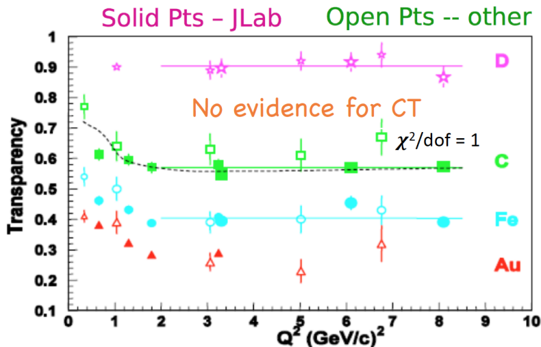
Figure 1: The combined results are shown for A(e, e'p) searches for CT at MIT-Bates, SLAC, and JLab. A fit is shown that indicates no significant rise consistent with CT. [29–31].
