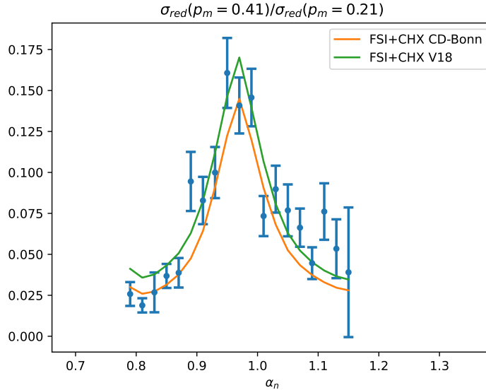
Figure 8: The reduced cross section ratio at Q^2 = 3.5 (GeV/c) ^2 is shown from the deuteron knockout experiment in [50] as a function of \alpha . While there is some difference in the choice of NN potential in describing the data, the difference is independent of Q^2 . Furthermore, these data are in agreement with the calculations in Fig. 7. Plot courtesy of W. Boeglin.
