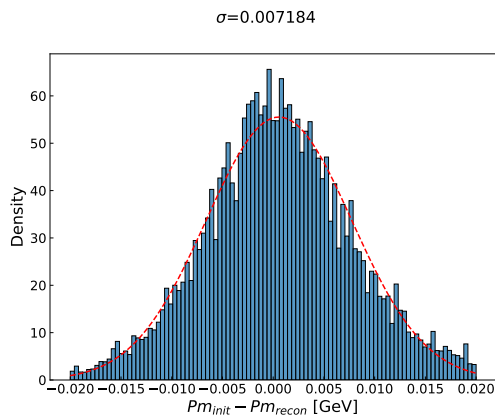
Figure 11: The P_m resolution at Q^2 = 14 \text{ (GeV}/c)^2 is about 7 MeV.
