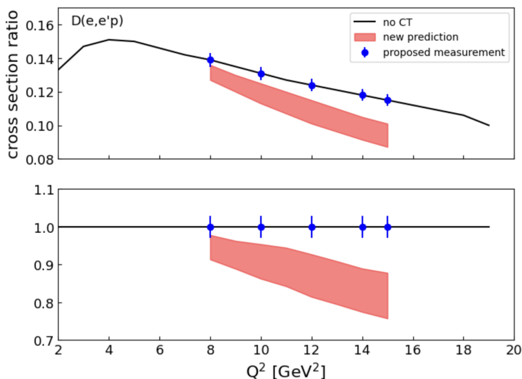
Figure 9: Here is the cross section ratio R = \frac{\sigma(p_r=400\text{MeV}/c)}{\sigma(p_r=200\text{MeV}/c)} in the d(e, e'p)n reaction (as from Fig. 7) overlaid with our proposed measurement. The shaded red band is the region between \Delta M^2=2-3 . The blue points are the kinematics in this proposal with their statistical uncertainty.
