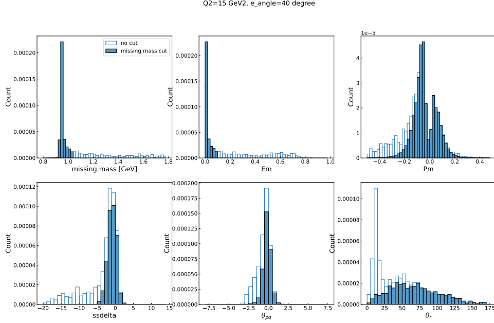
Figure 13: Kinematics variables from SIMC before (non-filled) or after (filled, blue) a missing mass cut of neutron mass \pm 0.1 GeV at Q^2 = 15 (GeV/c) 2 .
