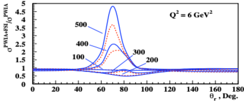
Figure 4: The dependence of the cross section ratio taken with respect to the PWIA on the recoil angle of the neutron ( \theta_r ) for different values of the recoil neutron momenta is shown for Q^2 = 6 (GeV/c) ^2 [47].
