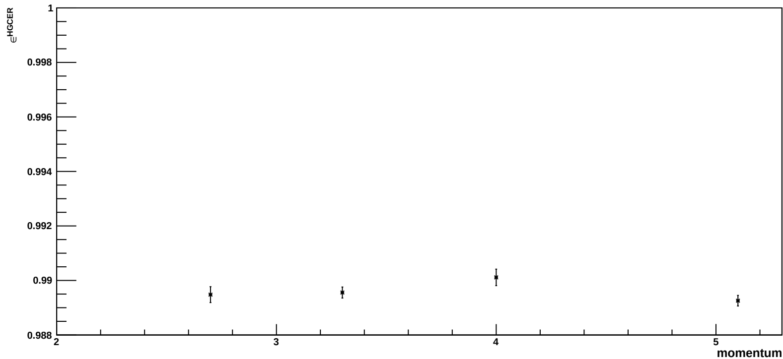
Hgcer Efficiency Vs Momentum
