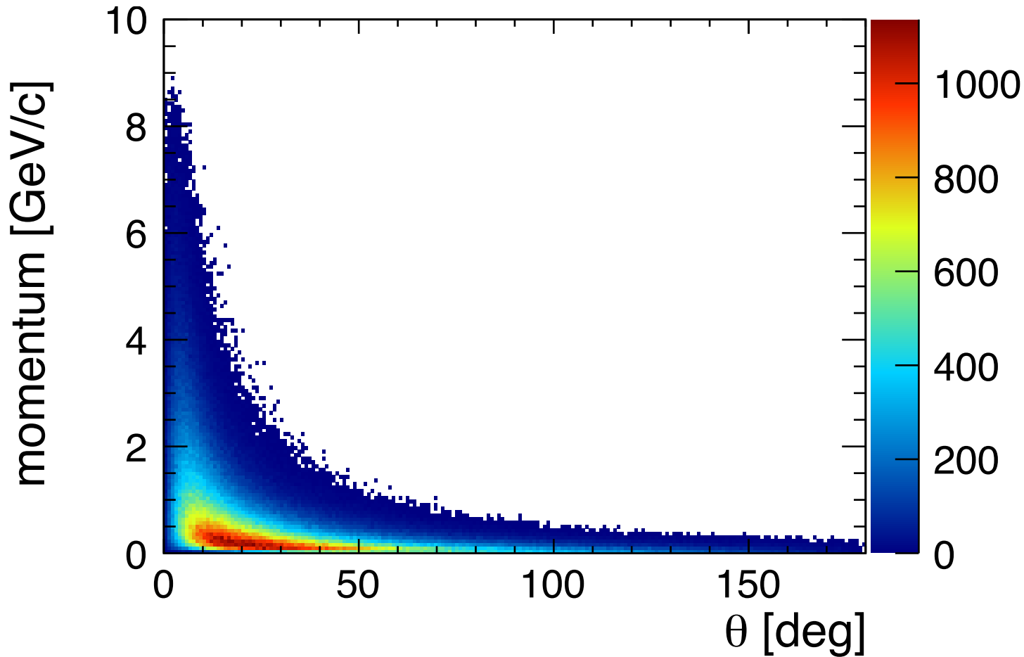
Thrown momentum vs. theta for gammas
