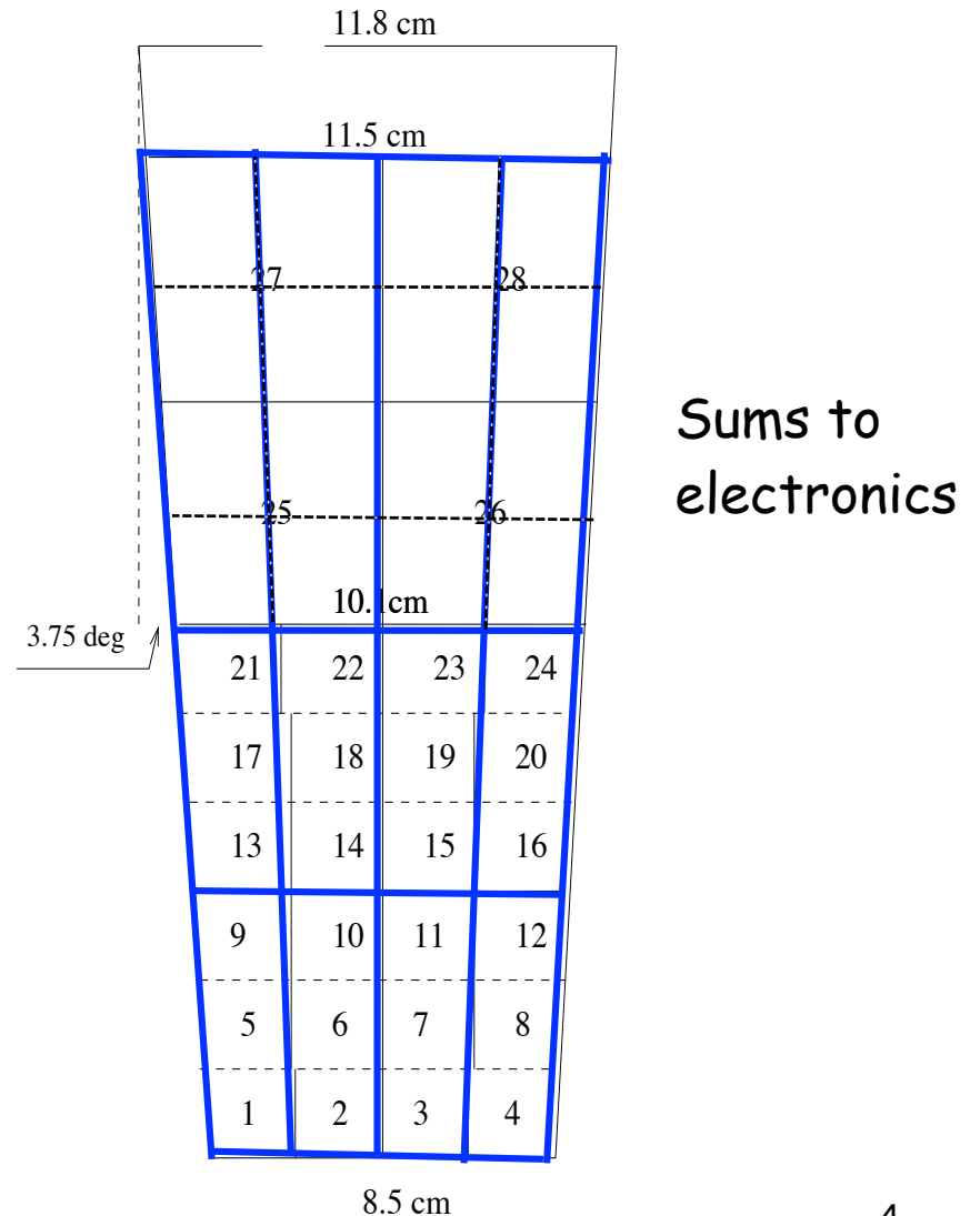
Conceptual layout for inner readout with SiPM
