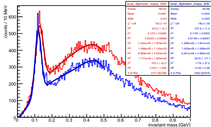
Old mcsmear Code (Red) and New mcsmear Code (Blue) [Shower Energy]
