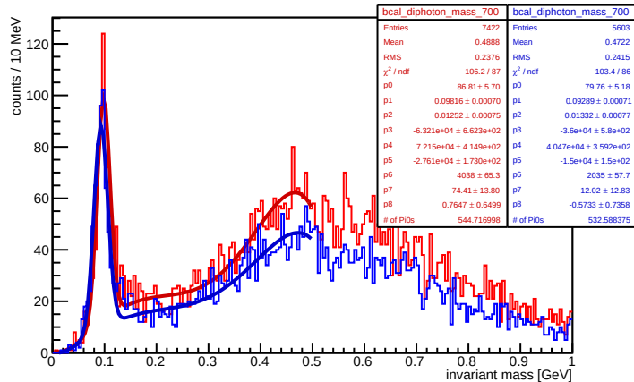
Old mcsmear Code (Red) and New mcsmear Code (Blue)
