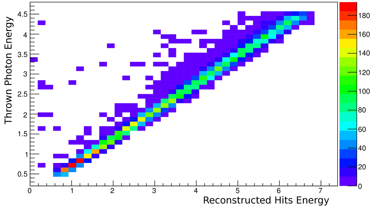
Thrown Energy vs. Reconstructed Energy
