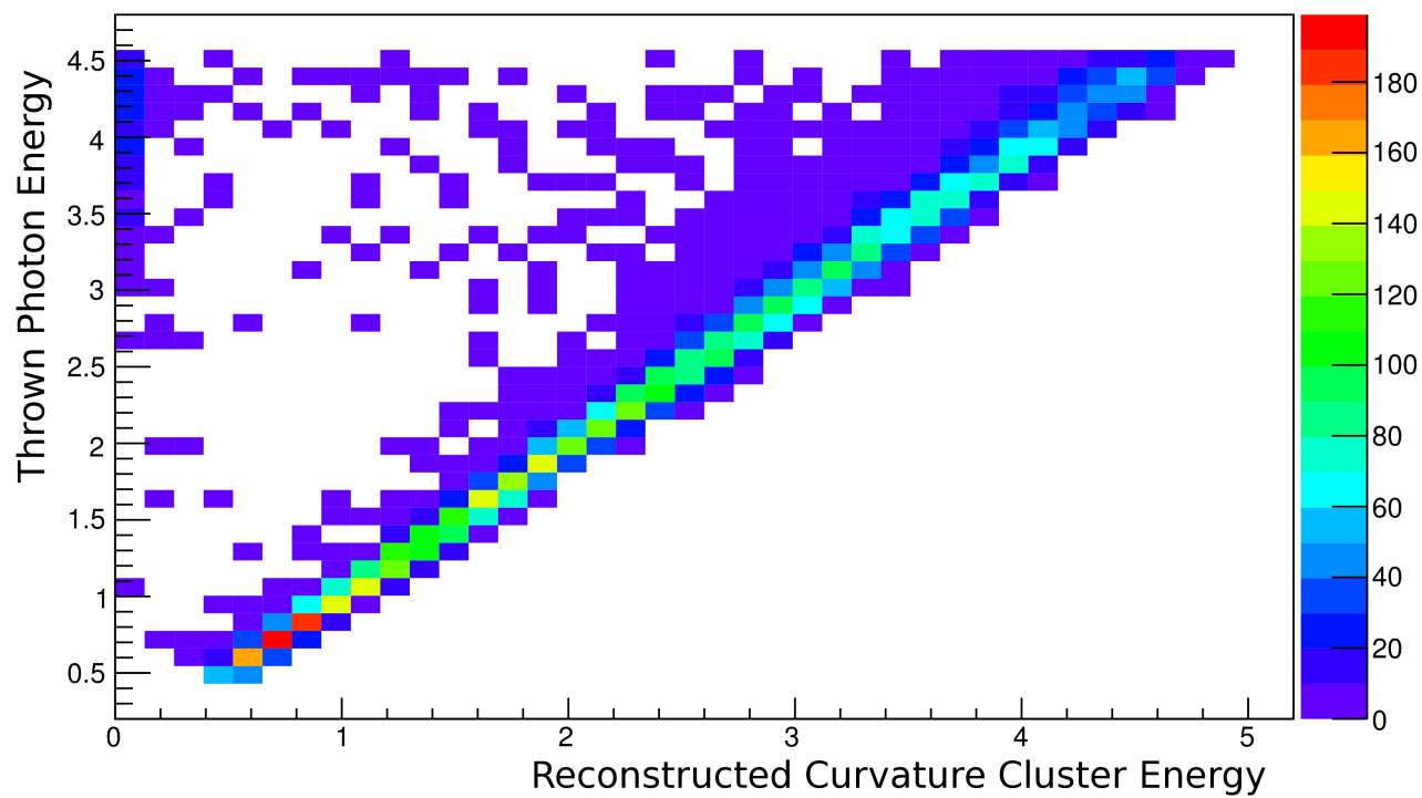
Thrown Energy vs. Reconstructed Energy
