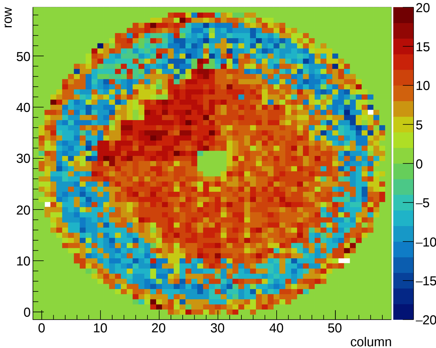
FCAL Timing Offsets (Run 31001)
