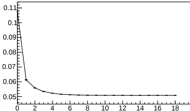
\sigma/\mu vs. Iteration (E1, E2 > 900 MeV)
