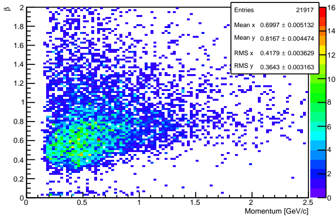
All PIDs, dNumParticleVotes>=2
