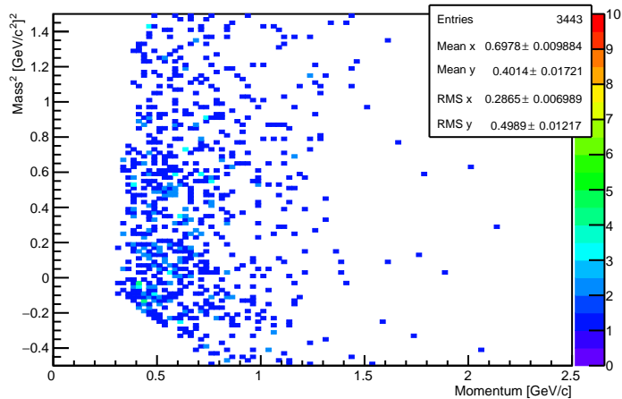
PID=14 (Proton), dNumParticleVotes>=2
