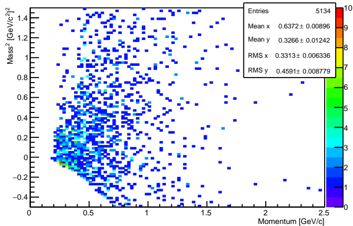
PID=11 (K+), dNumParticleVotes>=2
