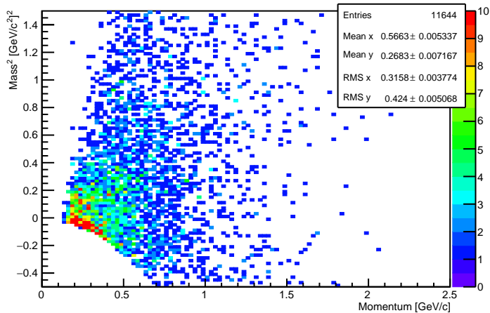
PID=8 (Pi+), dNumParticleVotes>=2
